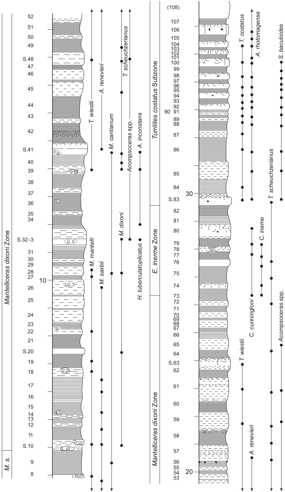
Text-fig. 9. The succession, and selected ammonite occurrences across the Lower-Middle Devonian boundary in the Southern Pit
