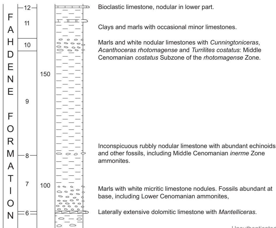
Text-fig. 7. The Lower/Middle Cenomanian boundary sequence south of Sif et Tella, Djebel Mrhila, Central Tunisia
