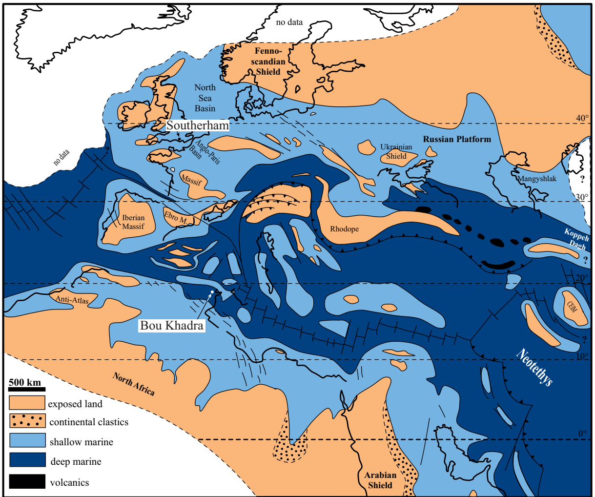
Text-fig. 2. The Cenomanian palaeogeography of the western Tethys (modified after Philip and Floquet 2000)
