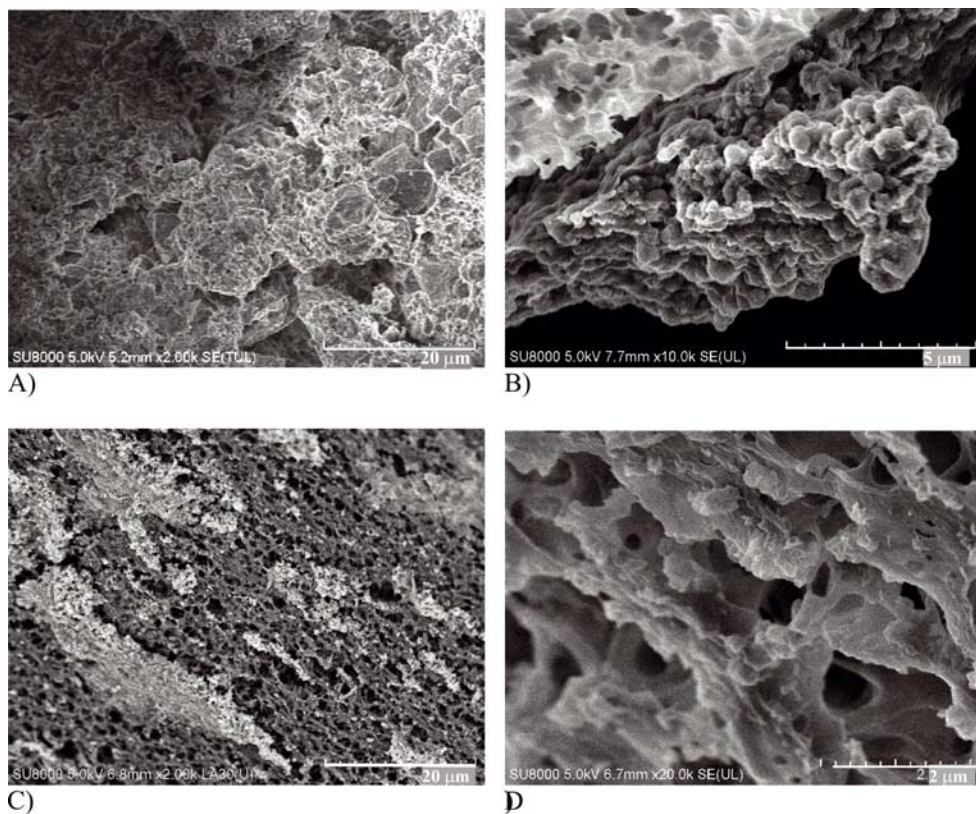
Figure 10. SEM images of membrane samples from collected MK4 module after 1200 h of MD process (330 K). A) inner surface (lumen side) 5 cm from module inlet, B) membrane cross-section with deposit, C) inner surface (lumen side) 15 cm from module inlet, D) magnified area from image C
