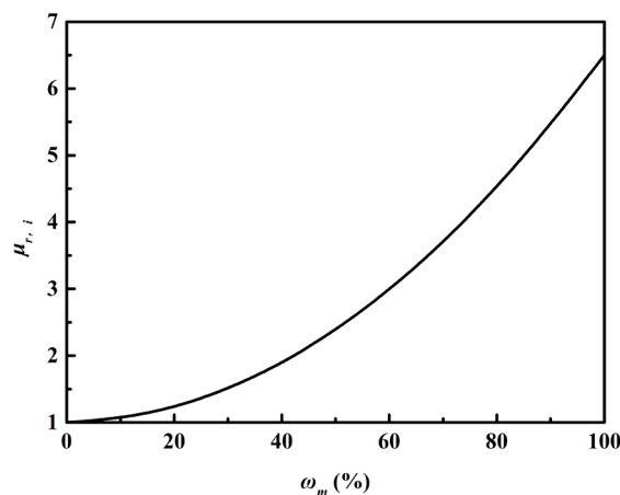
Fig. 6. The relationship between the relative permeability of interlocked particles and the volume percentage of magnetite
