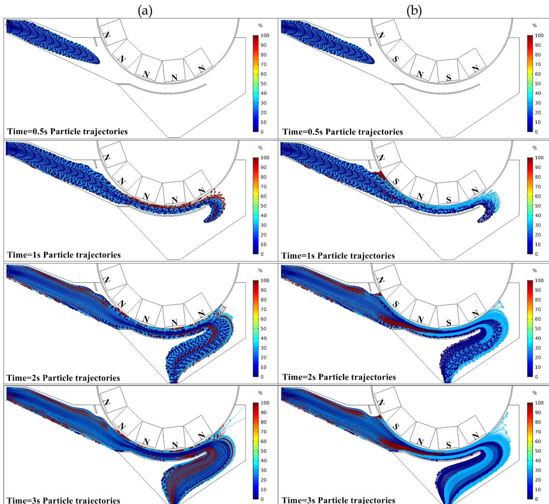
Fig. 4. 2D dynamic behavior of MTMPs in wet LIMS, where t = 0.5, 1, 2, 3 s. Particles are colored by the percentage magnetite content, and streamlines represent particle trajectories. (a) and (b) show the same information except for CMP and AMP
