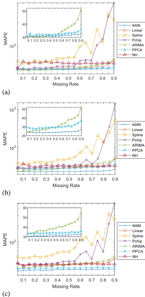
Fig. 8. The values of MAPE obtained by a set of imputing algorithms for (a) PeMS data set, (b) Portal data set, (c) Beijing data set
