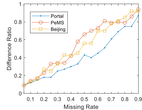
Fig. 4. Difference ratios (the number of the unique order of k nearest neighbours over 100 independent runs) for each missing rate for the three data sets
