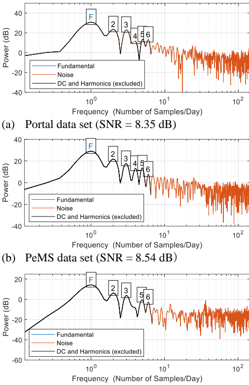
(a) Portal data set (SNR = 8.35 dB) (b) PeMS data set (SNR = 8.54 dB) (c) Beijing data set (SNR = 3.53 dB) Fig. 3. The power spectrums of the traffic flows for the three data sets
