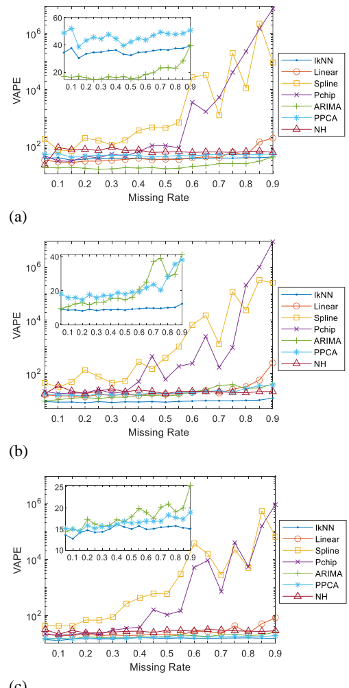
Fig. 9. The values of VAPE obtained by a set of imputing algorithms for (a) PeMS data set, (b) Portal data set, (c) Beijing data set
