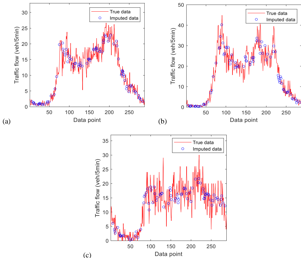
Fig. 6. The imputed results for (a) PeMS data set, (b) Portal data set, (c) Beijing data set, with missing rate of 0.7
