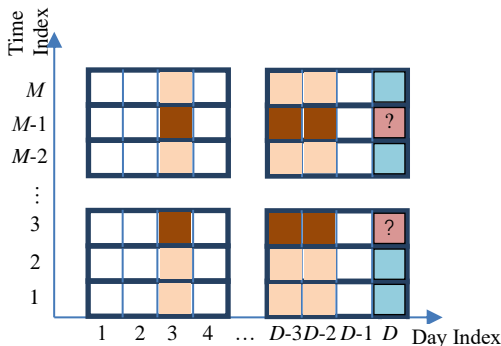
Fig. 1. Illustration of the kNN algorithm used to impute the data
