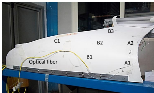
Fig. 7. FBGs points map on the composite winglet
