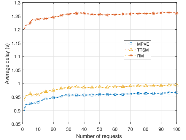
Fig. 5. Average delay versus the number of requests.
