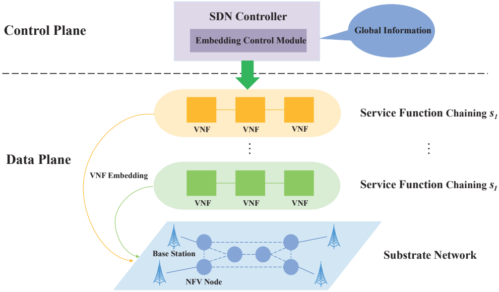
Fig. 1. VNF embedding for SDN-enabled PD-IoT framework.
