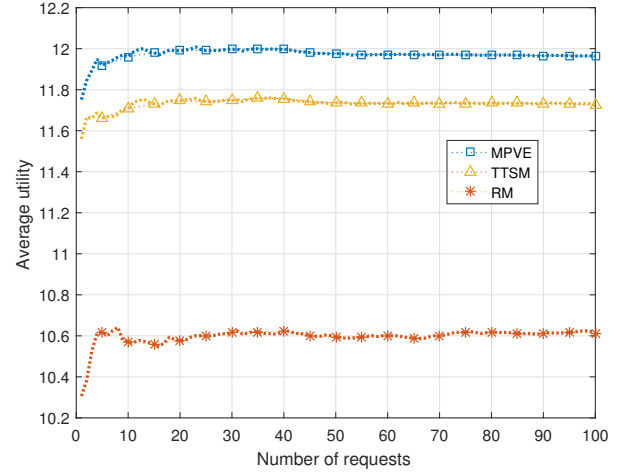
Fig. 2. Average utility versus the number of requests.
