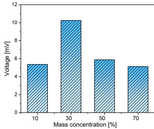
Fig. 11. Histogram of backscattered equivalent voltage varying with mass concentration.
