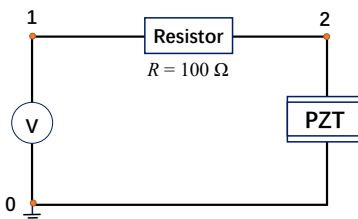
Fig. 6. Equivalent circuit diagram of the terminal.
