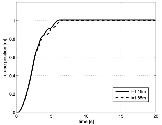
Fig. 9. Crane position – experiments for m = 50 kg
