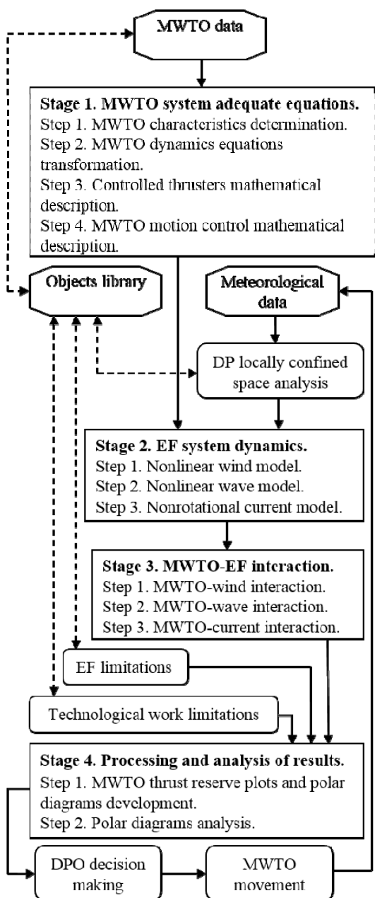
Figure 4. Information and logical model of methodology.
