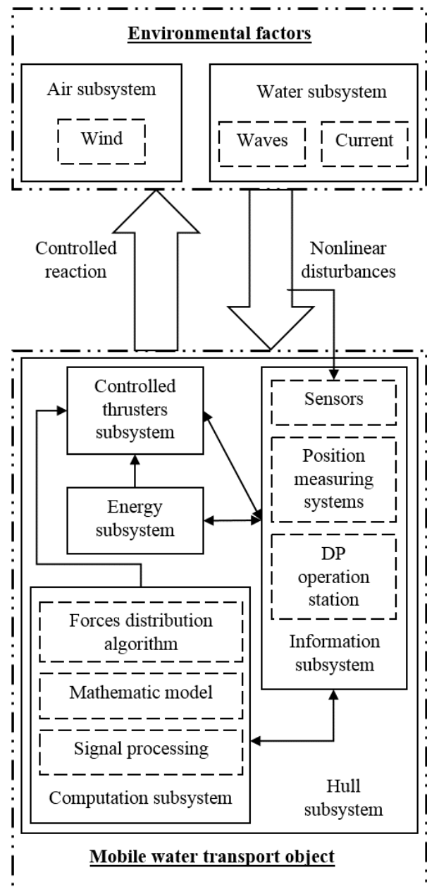
Figure 3. MWTO-EF systems complex interaction.
