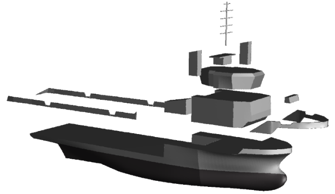
Figure 7. MWTO elements exposed to wind influence.
