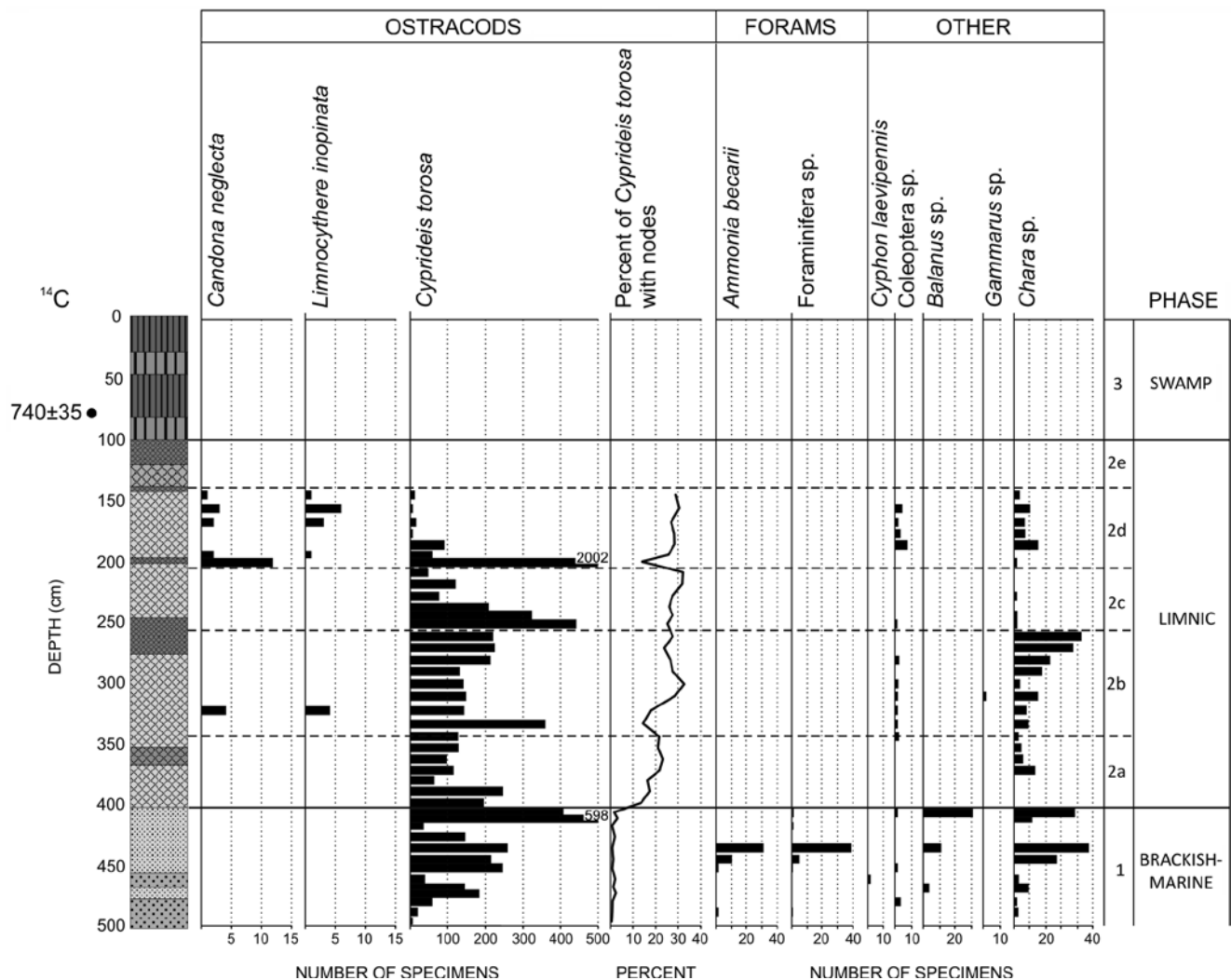
Fig. 5. Absolute frequency diagram of other micro- and macrofossils (absolute number of specimens) in the section Leb 1. Lithological signatures as in Table 1.
