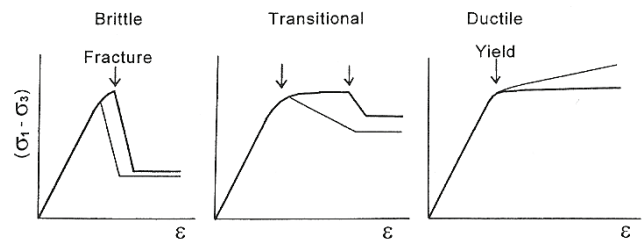
Fig. 1. Schematic representation of transition from brittle state to ductile flow depending on test confining pressure (after Mogi [16])
