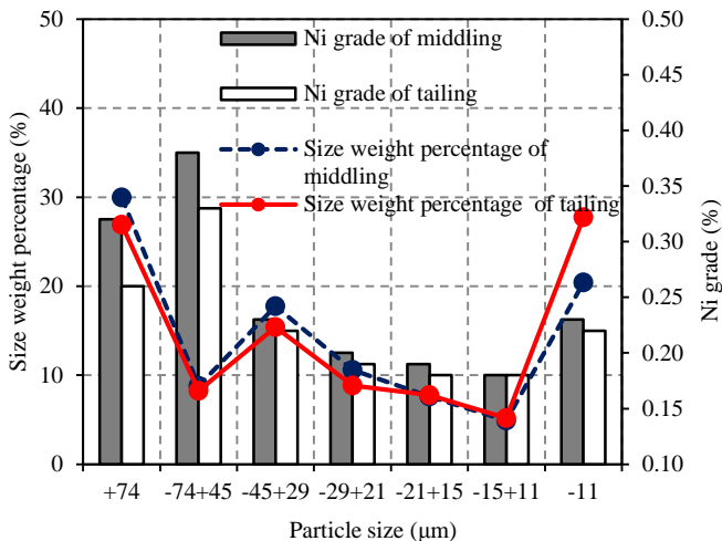
Fig. 3. Size analysis of circulating middling and tailing
