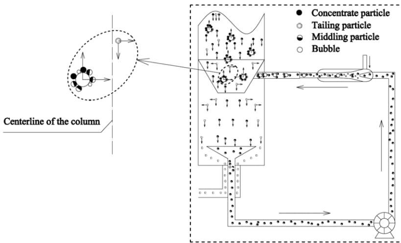
Fig. 2. Mechanism of cyclonic separation in the cyclonic flotation column
