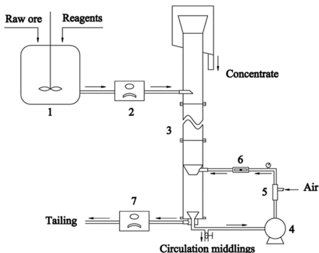
Fig. 1. Schematic illustration of the lab-scale cyclonic flotation column system. 1 mixing tank, 2 feed peristaltic pump, 3 column body, 4 circulation pump, 5 bubble generator, 6 gas flowmeter, 7 tailing peristaltic pump
