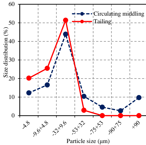
Fig. 5. Size distribution of chalcopyrite in circulating middling and tailing
