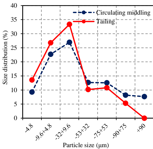
Fig. 4. Size distribution of pentlandite in circulating middling and tailing
