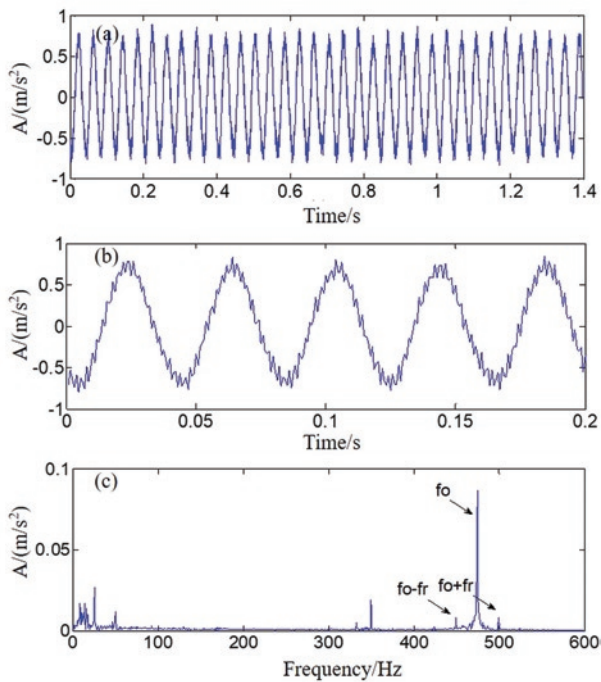
Fig. 11. The analysis of denoising results of NLM in case study 2: (a) denoising signal, (b) local amplification of the denoising signal and (c) envelope spectrum of denoising signal
