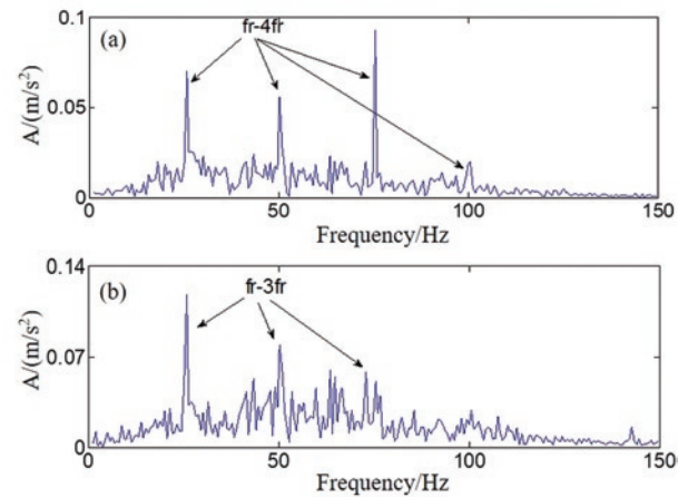
Fig. 9. The frequency spectra of fault component: (a) NLM and (b) Wden
