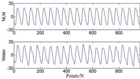
Fig. 3. The comparison of denoising results of two methods for simulation signal 1
