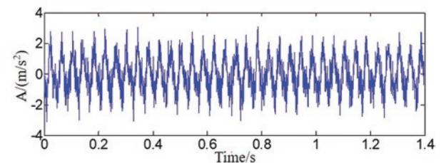
Fig. 10. The vibration signal of multistage centrifugal pump with bearing fault
