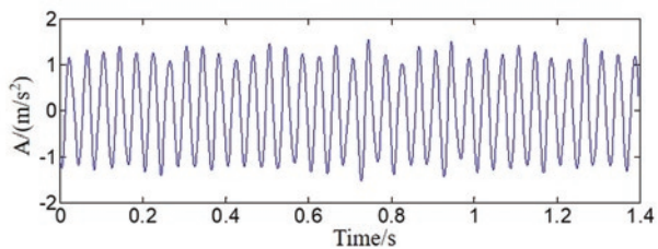
Fig. 12. The results of Wden in case study 2
