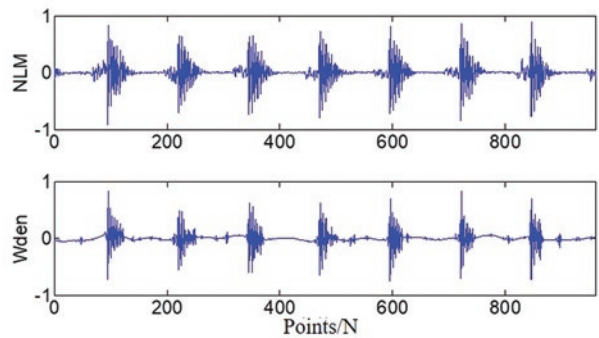
Fig. 5. The comparison of denoising results of simulation signal 2 for two methods
