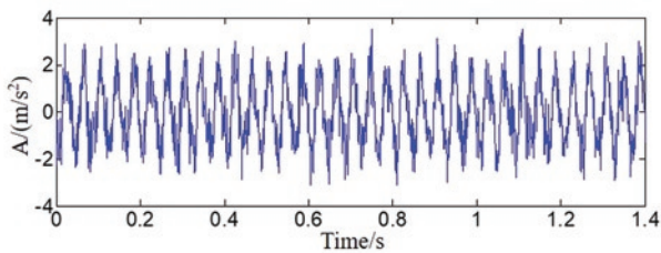
Fig. 7. The vibration signal of multistage centrifugal pump with misalignment
