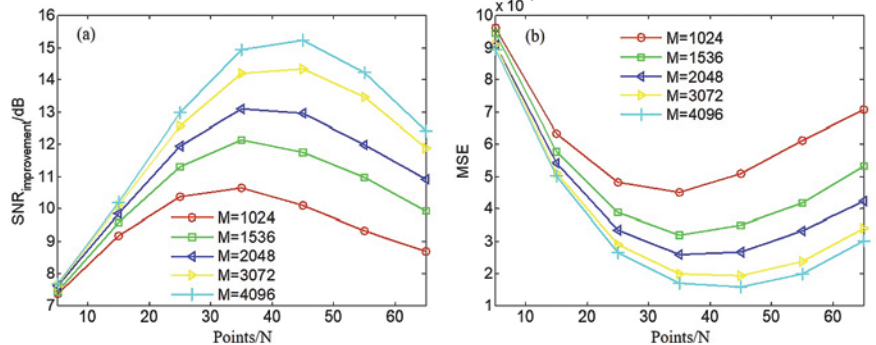
Fig. 6. The improvement of evaluation indicators versus P and M ( \lambda = 0.6\sigma ): (a) SNR improvement, (b) MSE
