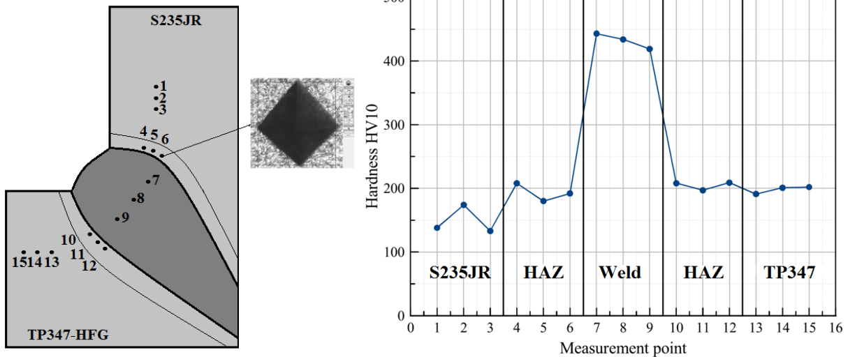
Fig. 8. Hardness distribution in cross-section of weld
