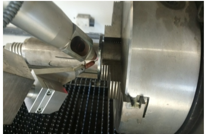
Fig. 6. Circumferential laser welding offlange filler joint
