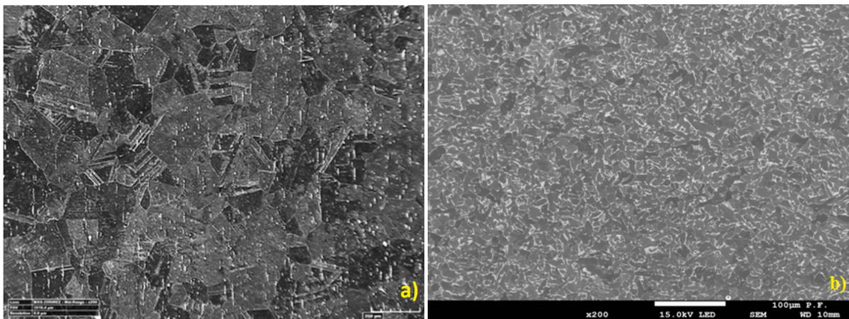
Fig. 9. BM microstructure: a) TP347-HFG, b) S235JR, magnification of ×200
