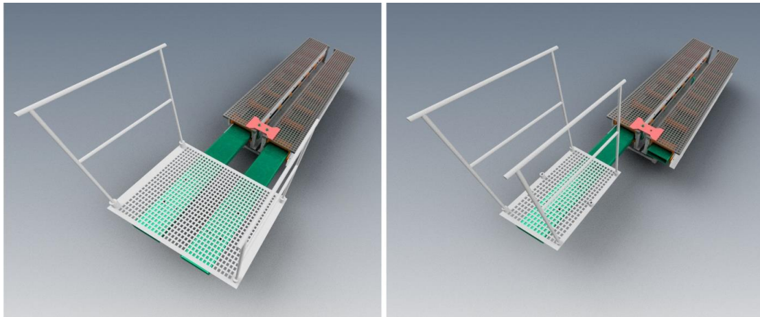
Fig. 2. A view of the mobile working platform unit equipped with different types of moveable platforms
