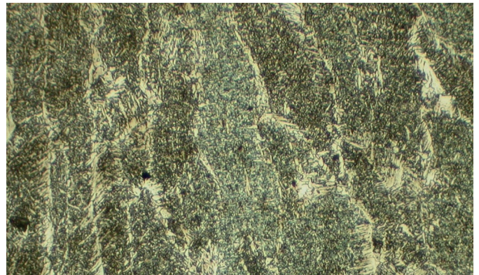
Fig. 3. Microstructure of WMD (63% of acicular ferrite) after MIG welding with micro-jet cooling of gas mixture (33% argon, 67% air), magn. 200x
