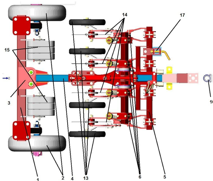
Fig. 6. General view of the technical system of operational monitoring of the state of the soil environment (top view)
