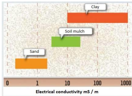
Fig. 1. Electrical conductivity of soil [17]
