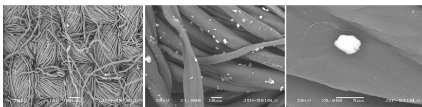
Figure 8. SEM photos of silver cyclohexane mono carboxylate applied cotton fabrics (100 \times , 1000 \times , 5000 \times ).
