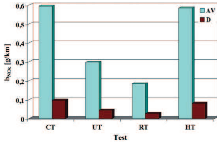
Fig. 12. The specific distance emission of nitrogen oxides - b_{NOx} at the PIMOT driving tests: AV - average value, D - standard deviation
