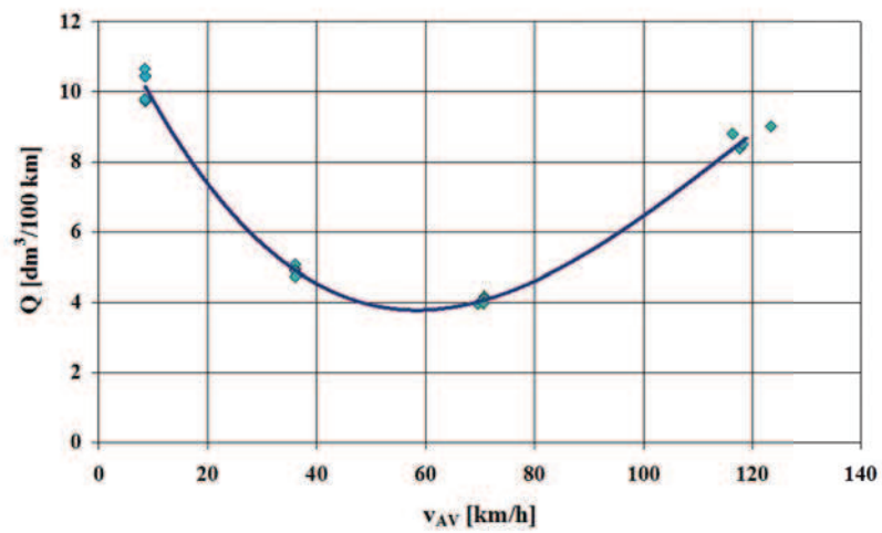
Fig. 21. Dependency of the operating fuel consumption - Q in the PIMOT driving tests on the average velocity - v_{AV}
