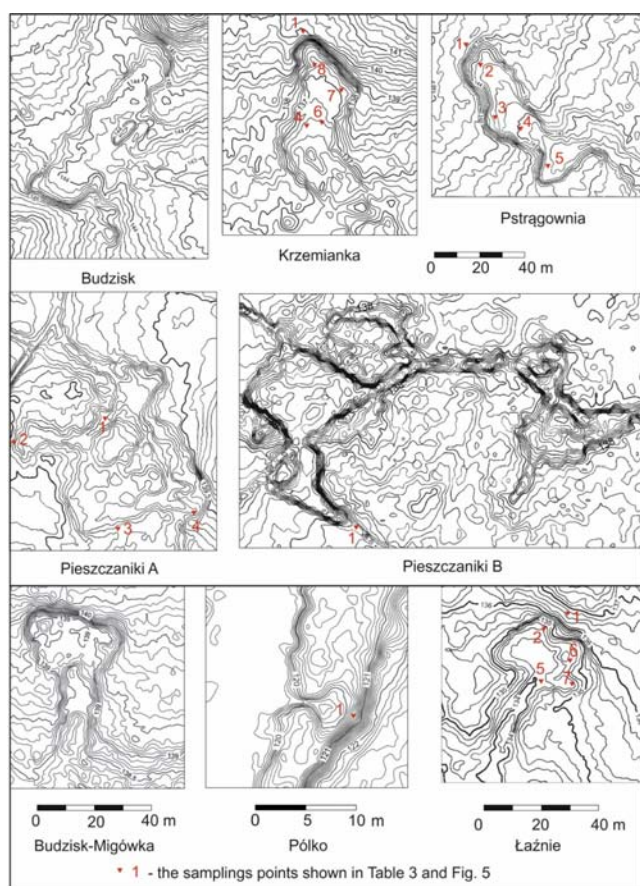
Fig. 6. Contour maps of selected spring-head alcoves; source: own study
