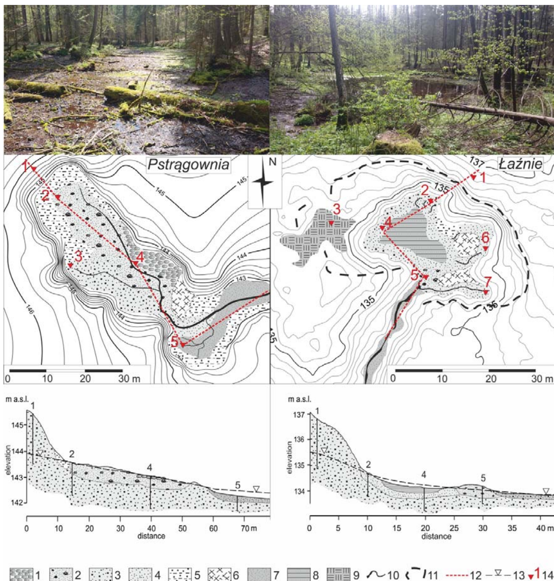
Fig. 4. The bottom deposits in the Pstrągownia and Łażnie spring-head alcoves; 1 = gravel-boulder erosional pavement, 2 = gravel with stones, 3 = medium sand with gravel, 4 = medium sand, 5 = colluvial sand of mixed grain size, 6 = deposits of the clumps and spurs, 7 = alluvial, fine-grained sand, 8 = fine-grained lake deposits with organic material, 9 = peat, 10 = watercourses, 11 = old edge of the alcove, 12 = cross section, 13 = watertable, 14 = samplings; source: own study
