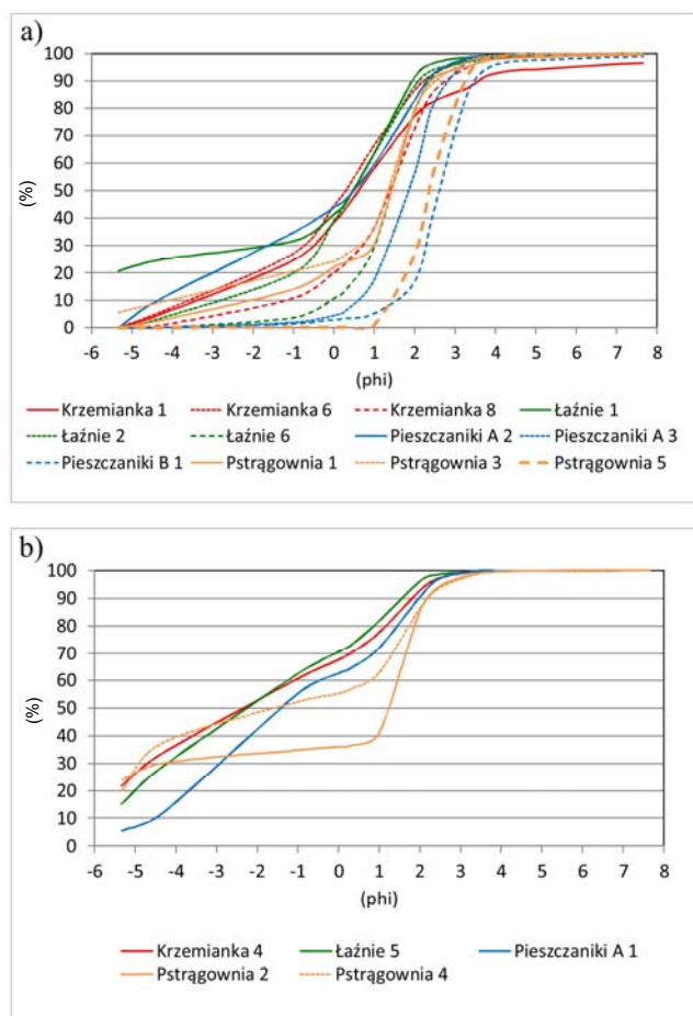
Fig. 5. Grain size distribution curves of the deposits of the selected spring-head alcoves in Knyszyńska Primeval Forest: a) aquifer deposits, b) bottom deposits; source: own study
