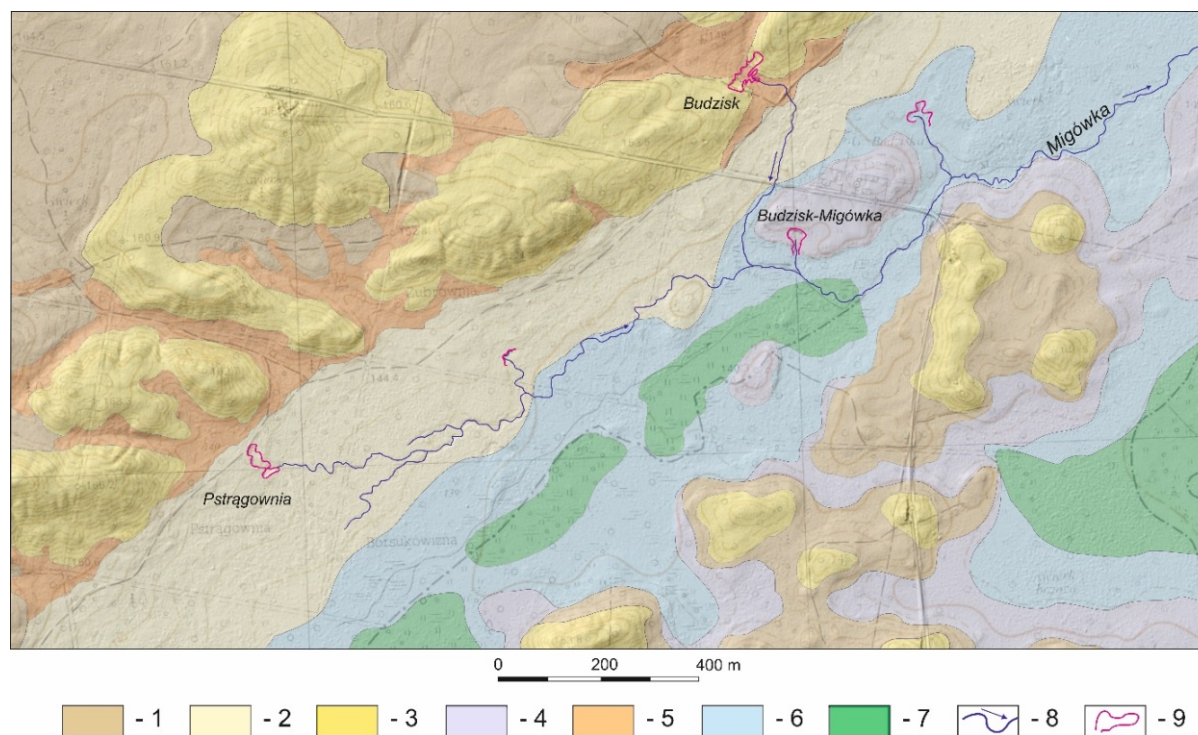
Fig. 2. Geological structure of Budzisk area (the Knyszyńska Primeval Forest), expanded the Warta Glaciation: 1 = ground moraine glacial sands and gravels with boulders, 2 = fluvio-glacial sands and gravels of outwash plains and outwash valleys, 3 = sands and gravels of kames, 4 = sands of meltout depressions; the Pleistocene/ the Holocene: 5 = colluvial sands and silt sands; the Holocene: 6 = peaty deposits on fluvio-glacial sands and gravels on the bottoms of valleys, 7 = peat, 8 = watercourses, 9 = spring-head alcoves; source: own elaboration based on LASKOWSKI [2000] and Geoportal [2017]
