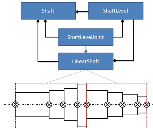
Fig. 10. Third shaft model.
