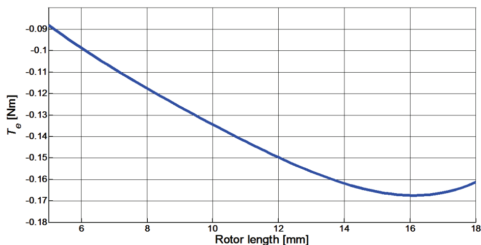
Fig. 12. Braking torque vs. rotor length at rated speed for the uniform rotor
