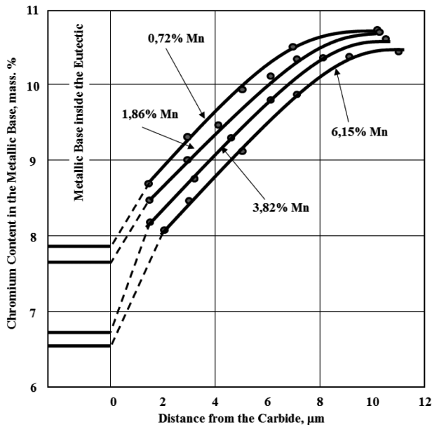
Fig. 3. Dependence of Cr content in the metallic base on Mn content and on the distance from carbides in the ЧX16HC cast iron
