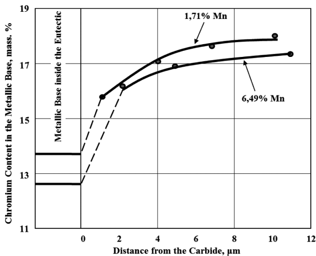
Fig. 4. Dependence of Cr content in the metallic base on Mn content and on the distance from carbides in the ЧX25C cast iron
