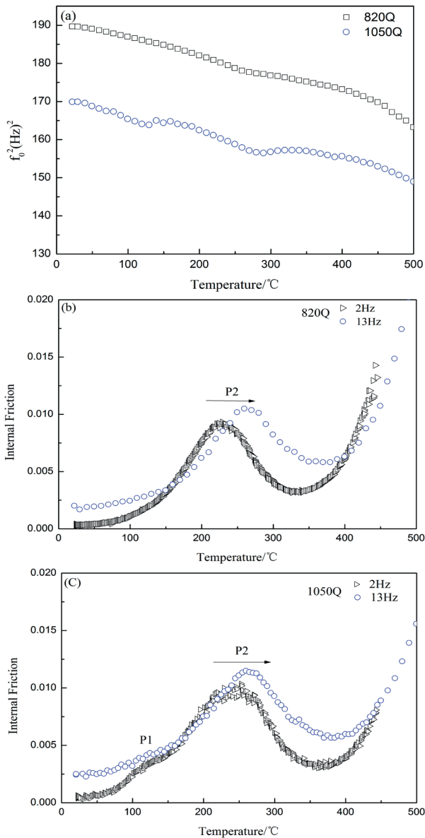
Fig. 2. (a) Temperature variation of Young's modulus ( E \sim f_0^2 ; where f_0 is the resonant frequency, f_0 \approx 13 Hz); (b) internal friction in 820Q, and (c) 1050Q samples
