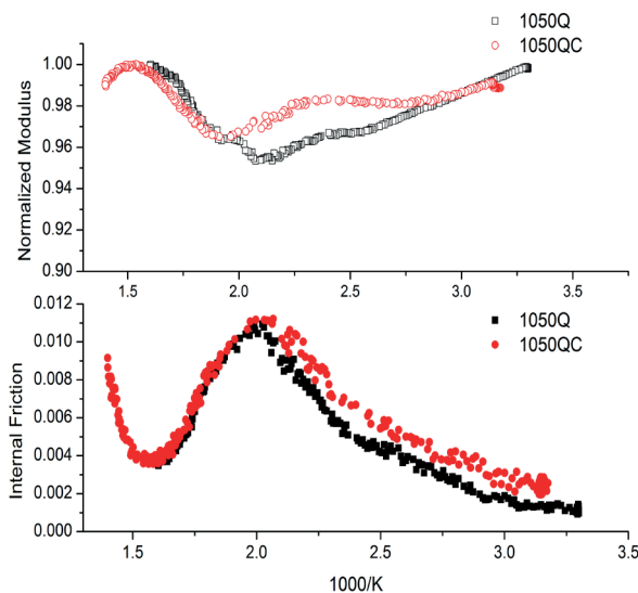
Fig. 5. Normalized modulus and internal friction spectra of 1050Q and 1050QC samples (the resonant frequency, f_0 \approx 2\text{Hz} )
