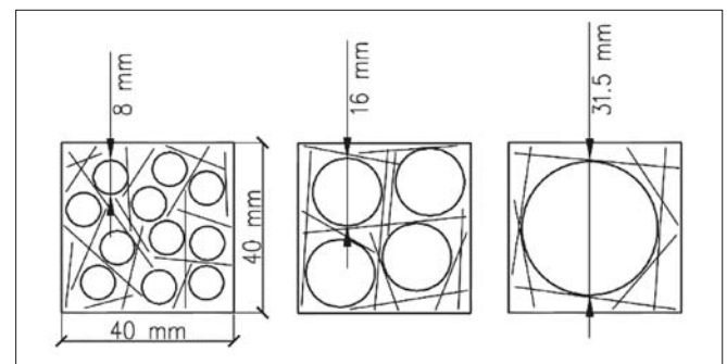
Fig. 6. Effect of fibre distribution according to size of aggregate
