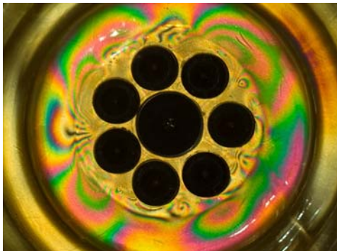
Fig. 1. Distribution of isochromatic on the surface of a damper hub model
