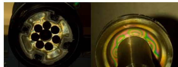
a) b) Fig. 16. Distribution of the effort of the registered as isochromatic on the surface of the damper: a - from the clamping screws, b - from the side of the crankshaft
