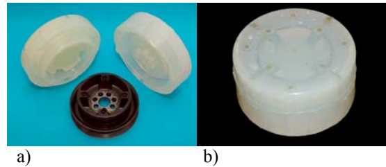
Fig. 5. The silicone mold of torsional vibration damper: a - the internal and external after separation, b - filled with an epoxy resin
