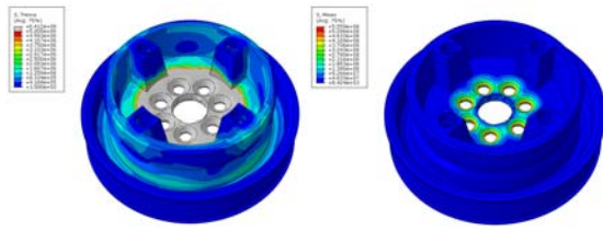
Fig. 17. Distribution effort of in the area of a damper hub mounting obtained by MES
