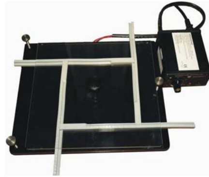
Fig. 8. Teflon plate for producing an optically active layer
