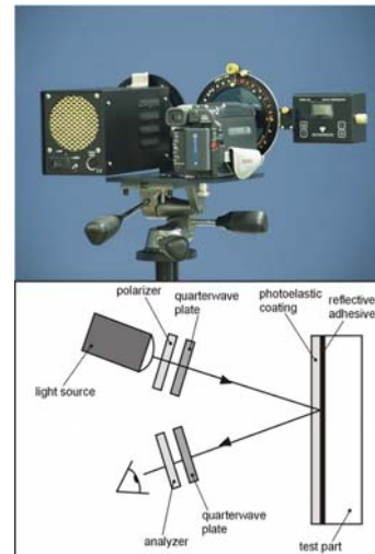
Fig. 2. Vishay polariscope on reflected light and the scheme of model by using polariscope
