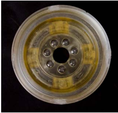
Fig. 7. Ready-made model of torsional vibration damper made from Epidian 5 epoxy resin
