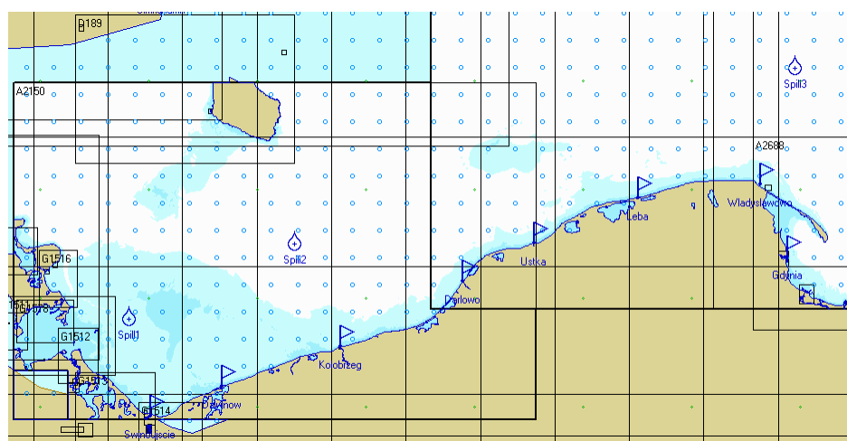
Fig. 4. Oil spills simulated positions[own study]
