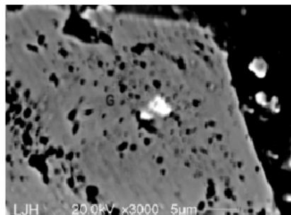
Fig. 3. Fine goethite (white) in magnetite mineral
