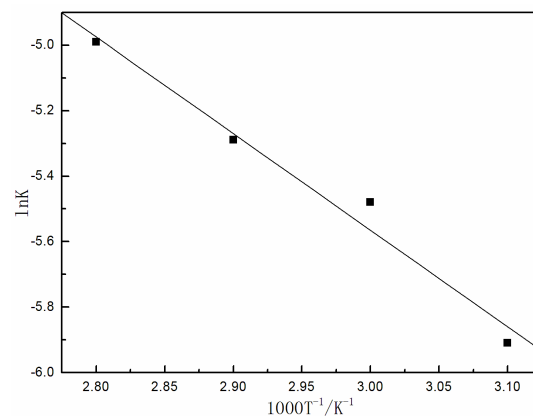
Fig. 13. The plot of \ln k-T^{-1} of manganese
