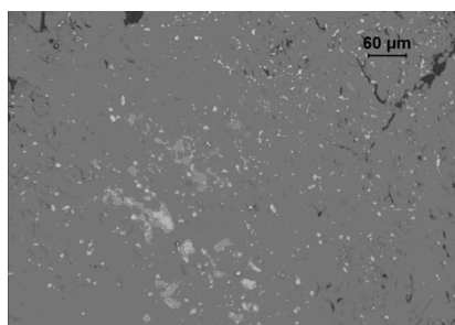
Fig. 4. Fine maghemite (white) and limonite (gray) located in gangue
