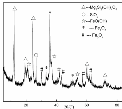
Fig. 2. Powder XRD pattern of raw laterite
