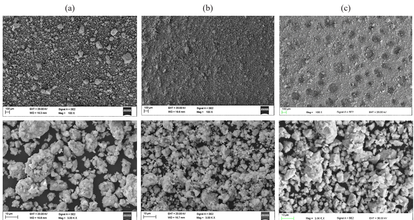
Fig. 3. Selected SEM micrographs showcasing the Mg 65 Zn 30 Ca 4 Er 1 alloy after a) 8, b) 13 and c) 20 hours
