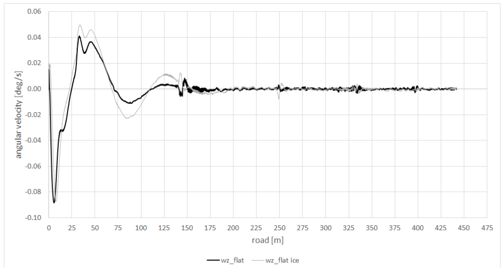
Fig. 25. Angular velocity around the vertical axis for the motion on a dry and icy flat road
