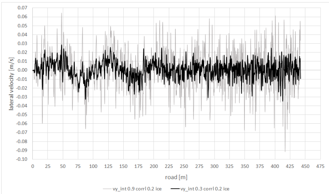
Fig. 14. Lateral velocity on an icy, randomly uneven road surface with the almost different left and right profiles of irregularities as well as different amplitudes of these irregularities
