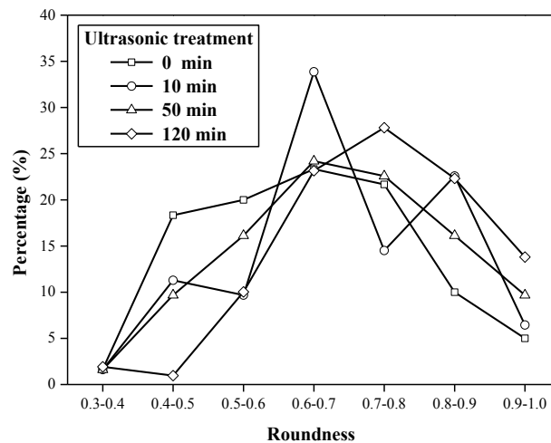
Fig. 7. Roundness distribution of 74-45 \mu\text{m} coal particles after 0, 10, 50, and 120 min ultrasonic treatment
