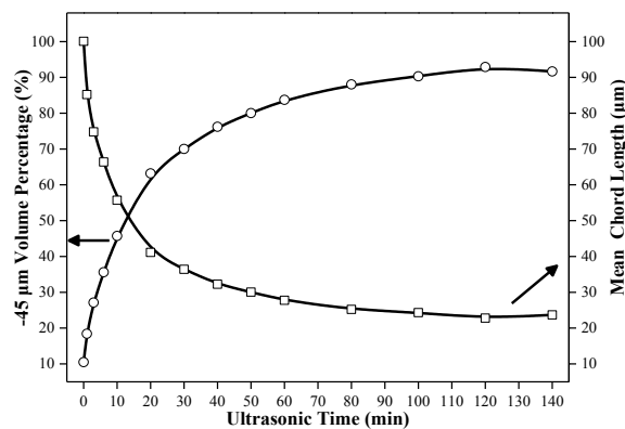
Fig. 4. Volume percentage of -45 \mu\text{m} coal particles and mean chord length of coal particles after ultrasonic treatment of different time (square-weighted)
