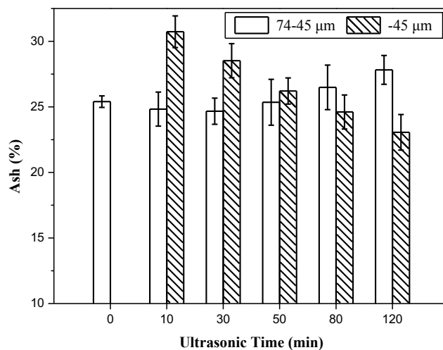
Fig. 8. Ash content of 74-45 \mu\text{m} and -45 \mu\text{m} size fractions after 10, 30, 50, 80 and 120 min ultrasonic treatment
