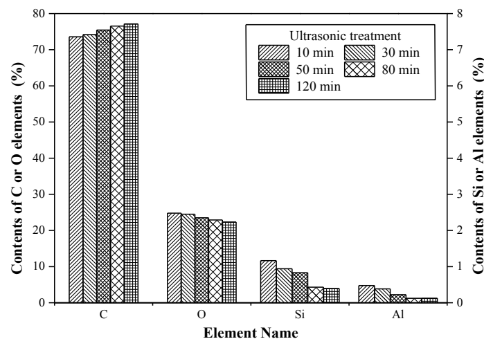
Fig. 11. Elements contents on -45 \mu\text{m} coal particle surfaces after 10, 30, 50, 80 and 120 min ultrasonic treatment
