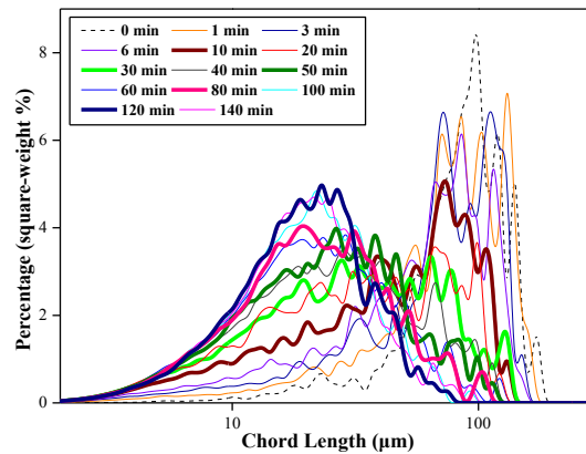
Fig. 3. Square-weighted FBRM chord length distribution of coal particles after ultrasonic treatment of different time
