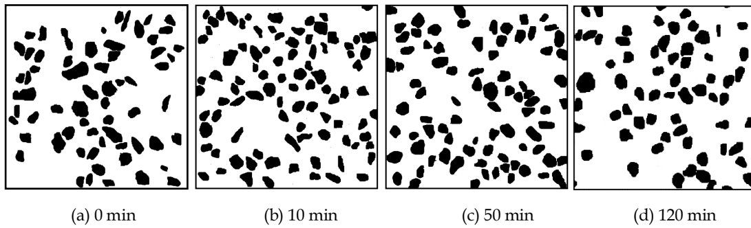
Fig. 6. SEM pictures of 74-45 \mu\text{m} coal particles after 0, 10, 50, and 120 min ultrasonic treatment after the image processing
