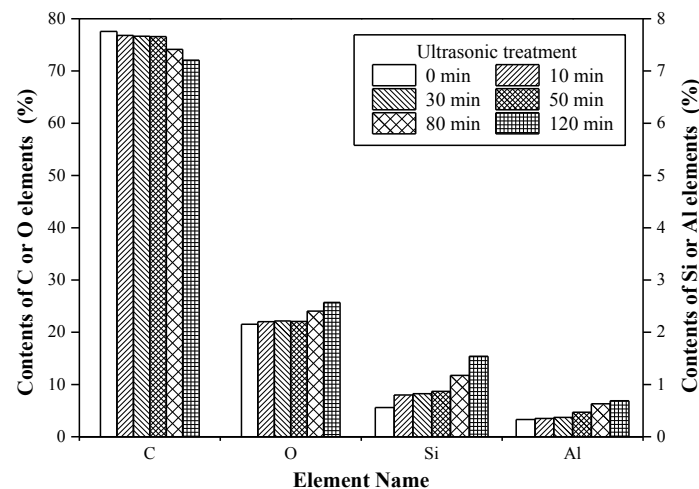
Fig. 10. Elements contents on 74-45 \mu\text{m} coal particle surfaces after 0, 10, 30, 50, 80 and 120 min ultrasonic treatment
