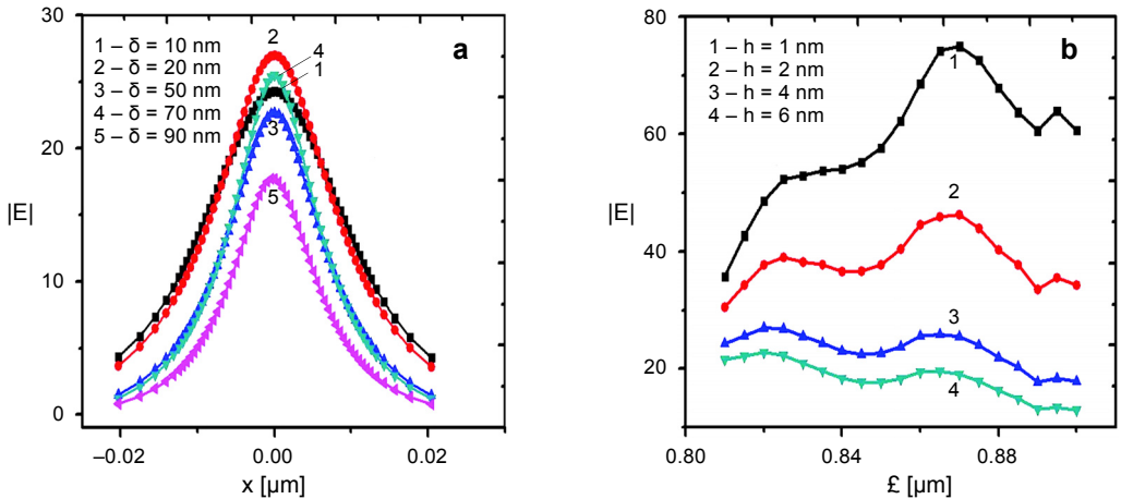
Fig. 5. The variations in electric field |E| as a function of the x for the different values \delta ; the frequency power monitors record the electric fields are located under the tip and the distance from the tip apex is h = 4 nm (a). Calculated variation in the electric field |E| as a function of probe tip model length \ell for different position h (b). The wavelength of incident light is 633 nm.
