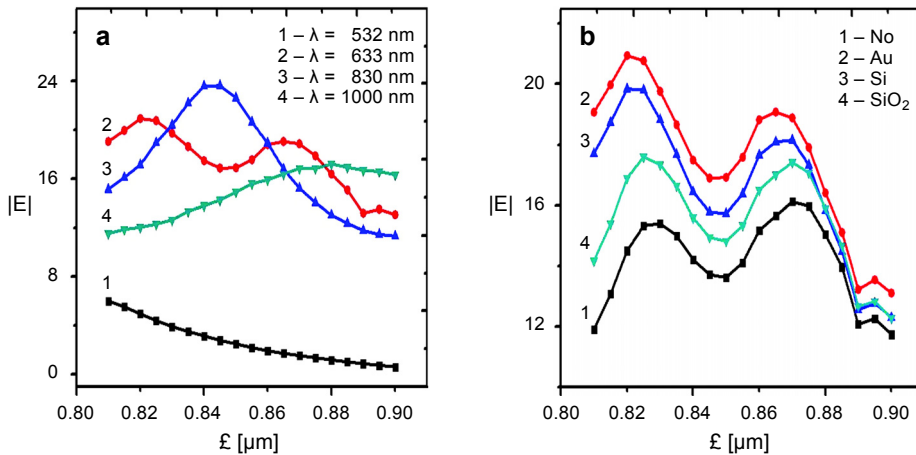
Fig. 6. The electric field enhancement |E| versus the probe length \mathcal{L} for different wavelength (the gold substrate) (a) and different substrate ( \lambda = 633 nm) (b). Most geometrical parameters are held constant; the ellipsoid protrudes from the truncated cone and the extension length is equal to the half-ellipsoid major axis, and \delta = 20 nm; the frequency power monitors position is h = 4 nm.
