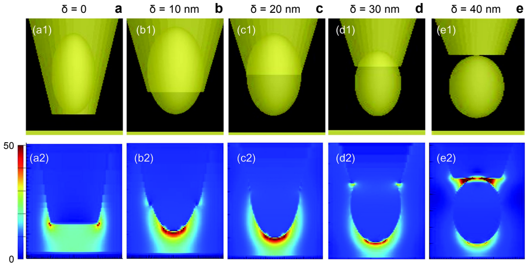
Fig. 2. The structures and the electric field distributions of the tip model in the x-z section for \delta = 0 (a), \delta = 10 nm (b), \delta = 20 nm (c), \delta = 30 nm (d), and \delta = 40 nm (e) of the ellipsoid protrude from the truncated cone.
