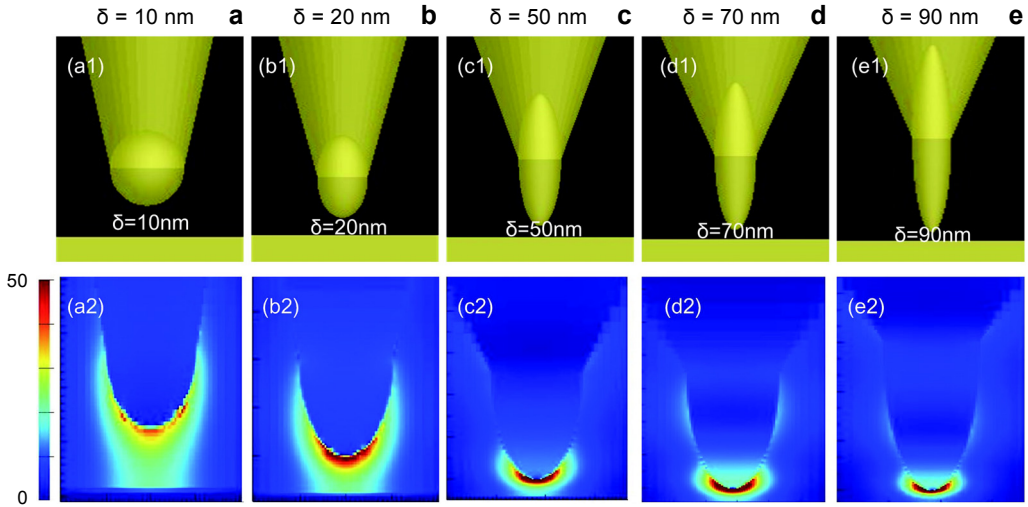
Fig. 4. The structures and the electric field distributions of the probe tip model. The ellipsoid protrude from the truncated cone and the extension length equal to the half-ellipsoid major axis. Most geometrical parameters are held constant, and the extension lengths are \delta = 10 nm (a), \delta = 20 nm (b), \delta = 50 nm (c), \delta = 70 nm (d), and \delta = 90 nm (e).
