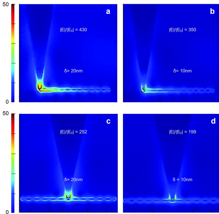
Fig. 7. Simulations of the electric field distribution for the tip at the left end ( a , b ) and the midsection ( c , d ) of the Ag nanowire, put on the \text{SiO}_2 substrate. The diameter and the length of the Ag nanowire are 10 and 1000 nm, respectively.
