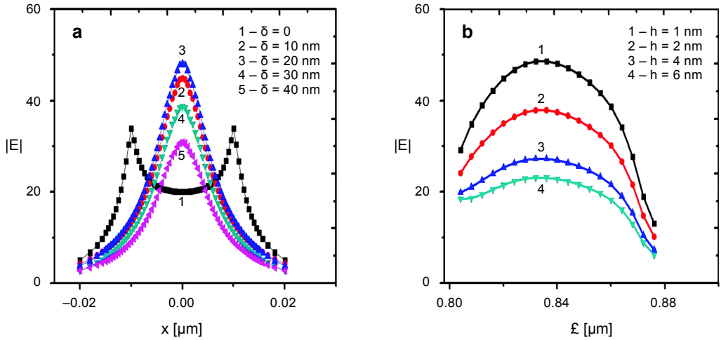
Fig. 3. The variations in electric field |E| as a function of the x for the different values \delta , and the frequency power monitors position is h = 4 nm (a). Calculated variation in the electric field |E| as a function of probe tip model length \ell for different position h (b). The length of minor and major axis of ellipsoid are d = 20 nm and j = 40 nm, respectively, and the wavelength of incident light is 633 nm.
