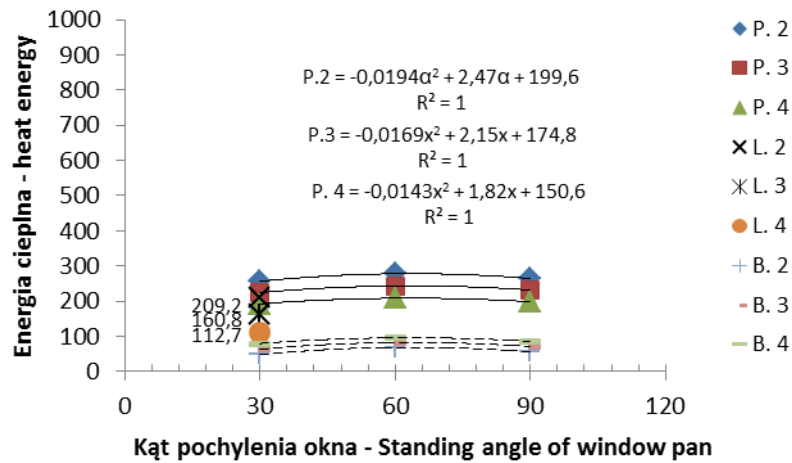
Fig. 2. Heat gains (P) and losses (L) and heat balance (B) depending on window angles and a number of panes in the winter period
