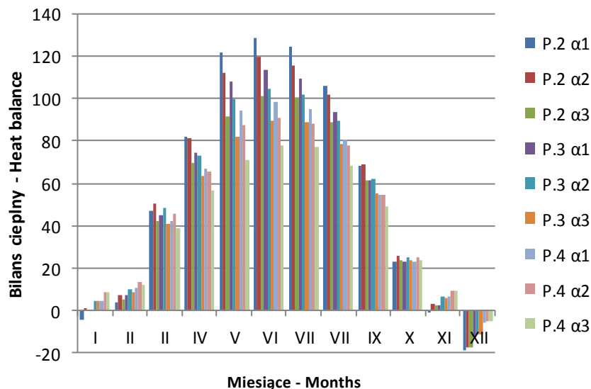
Fig. 3. Heat balance in consecutive months for a number of panes and window angles (notes: P – panes, 2, 3, 4 – a number of panes, α – window angle)
