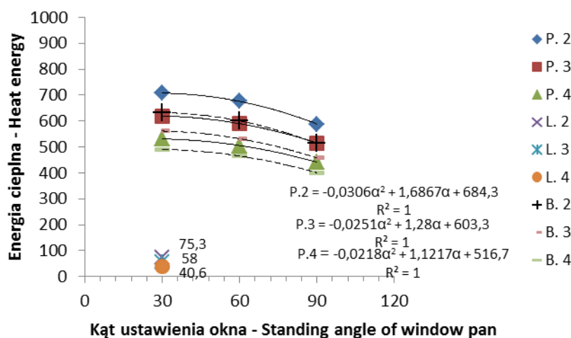
Fig. 1. Heat gains (P) and losses (L) and heat balance (B) depending on a window angle and a number of panes in the summer period
