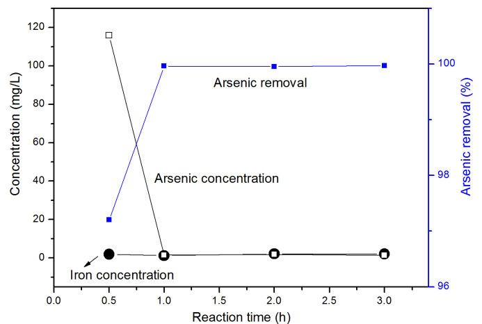
Fig. 3. As removal as a function of reaction time (initial As 4.13 g/L, temperature 70°C, H 2 O 2 /(2Fe + As) molar ratio = 1, Fe/As molar ratio = 1.5)
