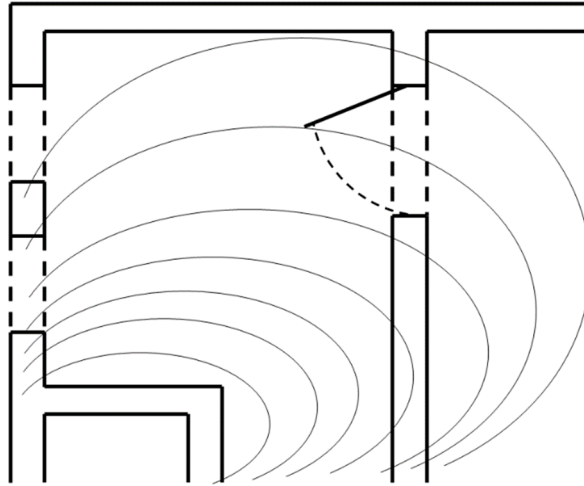
Figure 7. An example of the spectrum of the magnetic field inside a building. Own elaboration.
