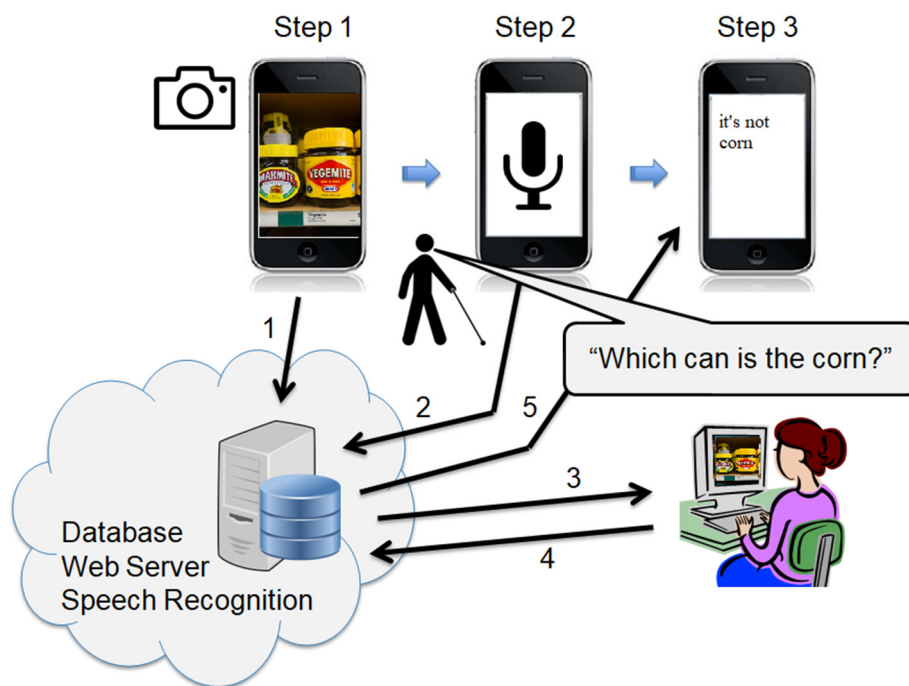
Figure 5. VizWiz– three steps algorithm that uses information to guide users to the appropriate object interactively from their phone. Own elaboration based on the sequence of messages and the architecture of the system presented in [2].
