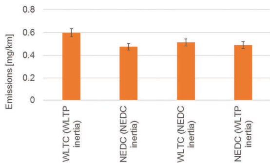
Fig. 13. PM emissions from vehicle 4 for the various test types performed
