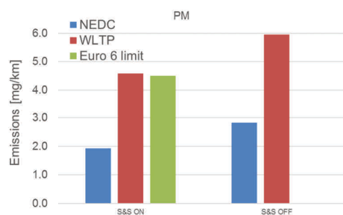
Fig. 1. PM emissions from vehicle 1
