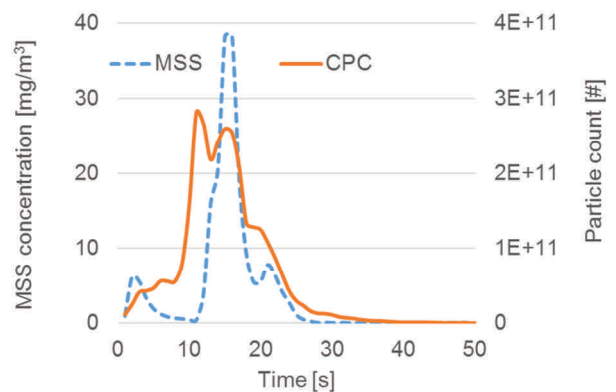
Fig. 11. CPC (solid particles only) and MSS readings over the first 50 seconds of the WLTP, for vehicle 3
