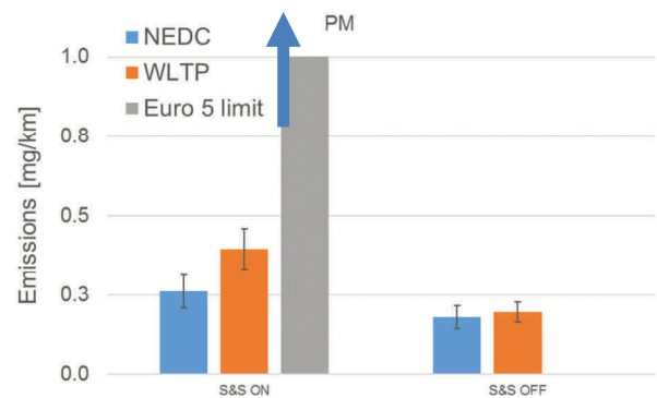
Fig. 5. PM emissions from vehicle 2. Note that the Euro 5 limit (4.5 mg/km) significantly exceeds the y-axis of the figure, being roughly ~10-~20 times the magnitude of the measured PM emissions
