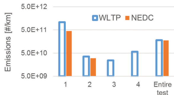
Fig. 9. PN emissions per phase and per test (solid particles only) for vehicle 3 (note that the NEDC consists of only two phases; note also the log 10 scale)
