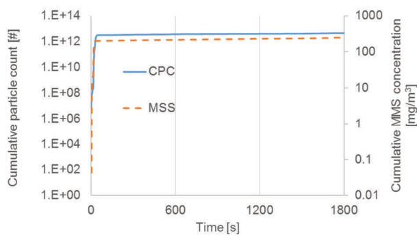
Fig. 10. Cumulative CPC (solid particles only) and MSS readings from vehicle 3 over the WLTP (note the \log_{10} scales on both vertical axes)
