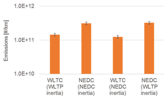
Fig. 14. PN emissions (solid particles only) from vehicle 4 for the various test permutations
