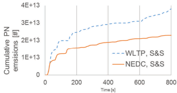
Fig. 3. Cumulative PN emissions (solid particles only) from vehicle 1
