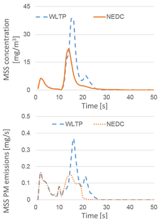
Fig. 12a: Raw MSS readings for the first 50 seconds of the NEDC and WLTP; and 12b: Calculated MSS emissions for the first 50 seconds of the NEDC and WLTP
