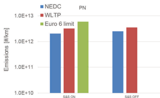
Fig. 2. PN emissions (solid particles only) from vehicle 1 (note the log 10 scale)
