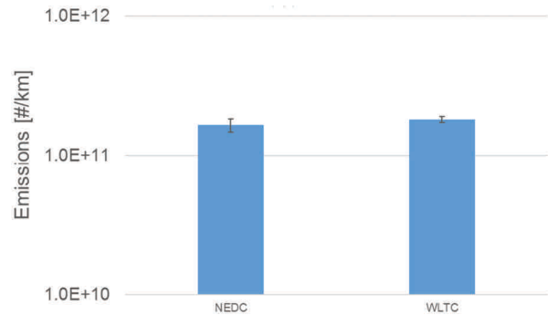
Fig. 8. PN emissions (solid particles only) from vehicle 3
