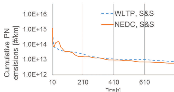
Fig. 4. Distance-specific cumulative PN emissions (solid particles only) from vehicle 1, calculated according to (2). The first 10 seconds have been excluded as distance-specific emissions during that period are \infty
