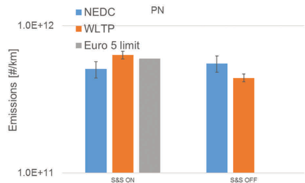
Fig. 6. PN emissions (solid particles only) from vehicle 2
