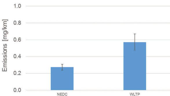
Fig. 7. PM emissions from vehicle 3
