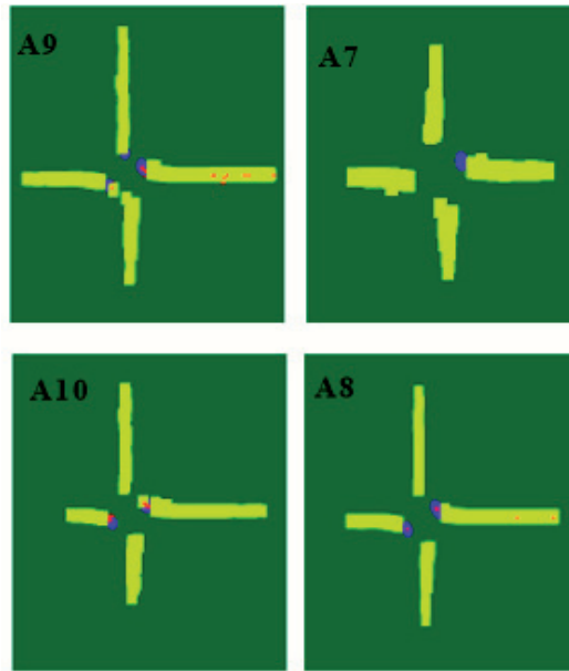
Fig. 9. Maps of potential conflicts in a Turbo roundabout created with SSAM
