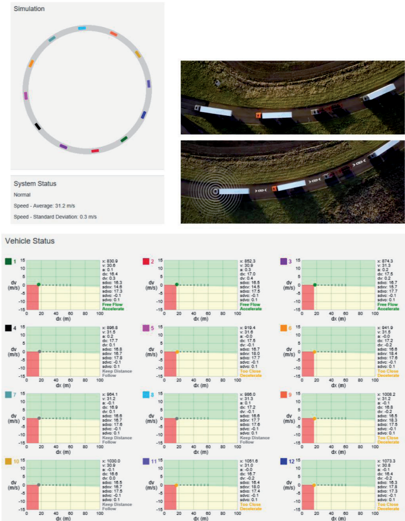
Fig. 7. W99 Car Following Model - How It Works for CAVs
