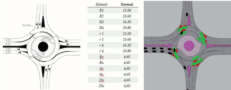
Fig. 1. layout of the turbo roundabout
