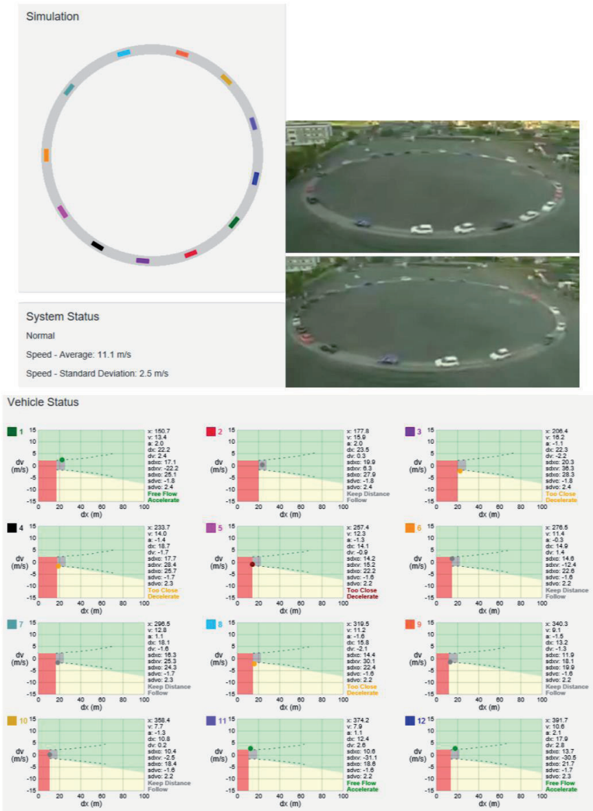
Fig. 6. W99 Car Following Model - How It Works for CVs
