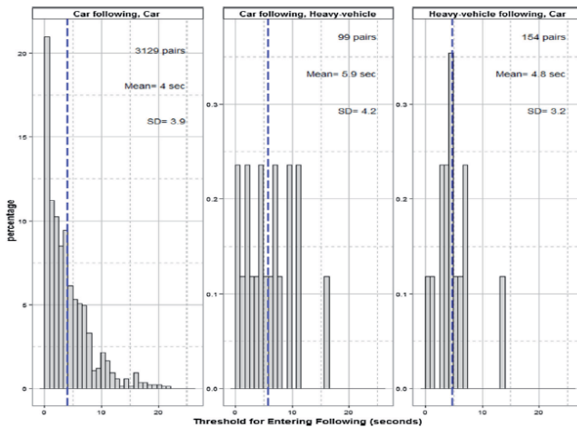
Fig. 5. Comparison of duration of the closing process among different vehicle-following cases
