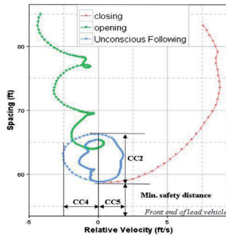
Fig. 3. CC2, CC4 and CC5 parameters from vehicle trajectory data
