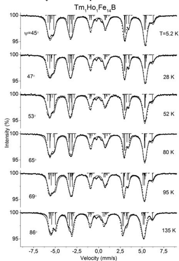
Fig. 1. The ^{57}Fe Mössbauer transmission spectra for Tm_1Ho_1Fe_{14}B (crosses – experimental data) and fits from the model (solid lines) illustrating the evolution of line positions and amplitudes. The change in lines of the 8j_2 sextet is visible. The angle \psi describing the rotation of magnetic moment and the temperature are indicated.
