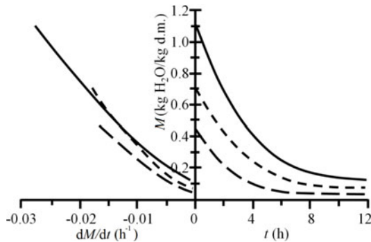
Figure 2. Moisture content vs. time and drying rate vs. moisture content for drying of sawdust at 60°C: (—) alder, (---) mixture of spruce and alder (60% and 40%, respectively), (- -) spruce
