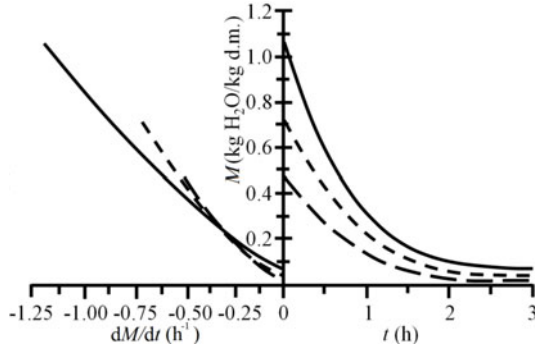
Figure 3. Moisture content vs. time and drying rate vs. moisture content for drying of sawdust at 150°C: (—) alder, (---) mixture of spruce and alder (60% and 40%, respectively), (- -) spruce
