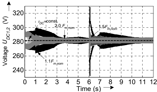
Fig. 6. DC-link capacitor voltages U_{DC1,2} for various control quality requirements
