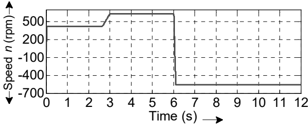
Fig. 3. Speed of the drive for F_m(t_k) < 1.5F_m \text{ nom}
