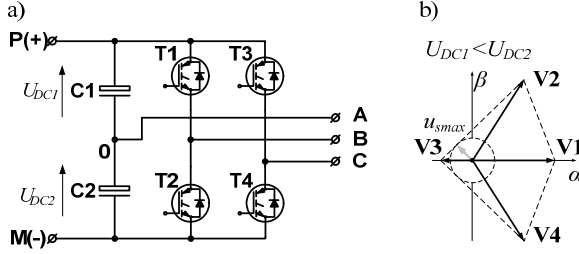
Fig. 1. Four-switch inverter topology (a) and a maximal voltage vector u_{s\text{ max}} under DC-link voltage imbalance (b)
