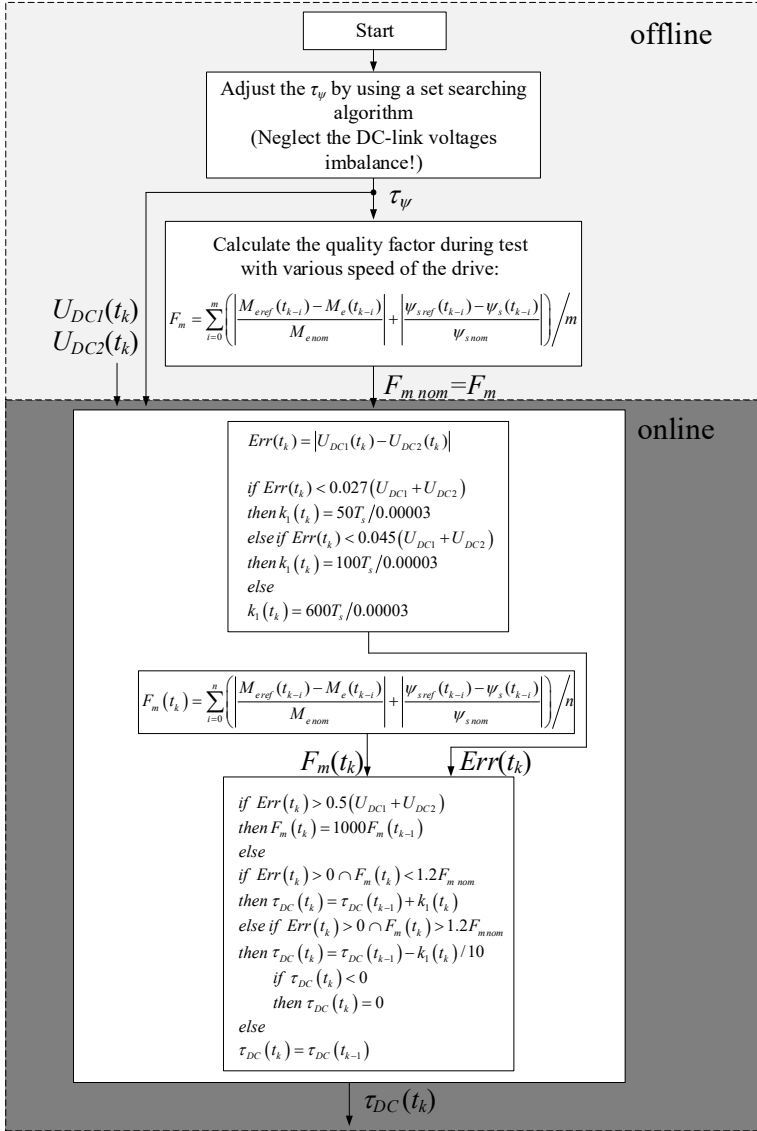
Fig. 2. Fitting procedure of weighting factors
