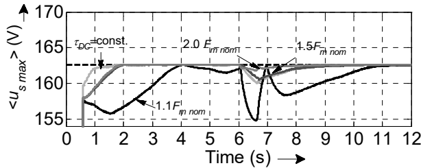
Fig. 7. Mean value of maximal inverter voltage u_{s\text{max}} that can be generated in linear modulation mode of the inverter for various control quality requirements
