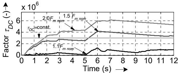
Fig. 5. Weighting factor \tau_{DC} for various control quality requirements
