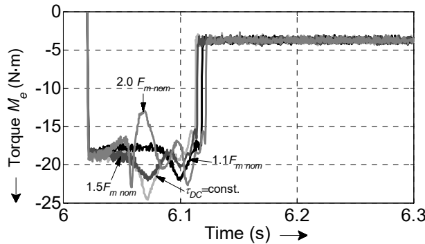
Fig. 8. Electromagnetic torque M_e during a rapid change of the motor speed for various control quality requirements
