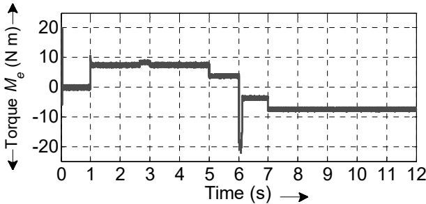
Fig. 4. Electromagnetic torque of the drive for F_m(t_k) < 1.5F_m \text{ nom}
