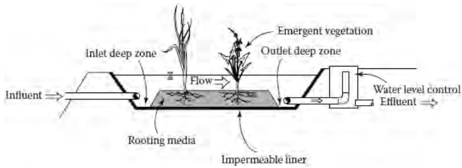
Fig. 10. Simple surface wetland; source: KADLEC and WALLACE [2009], modified
