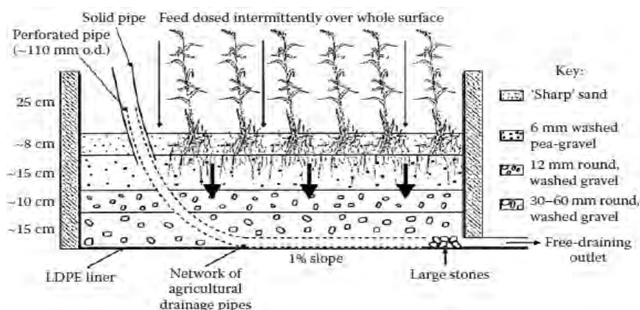
Fig. 14. Vertical flow wetland; source: KADLEC and WALLACE [2009], modified
