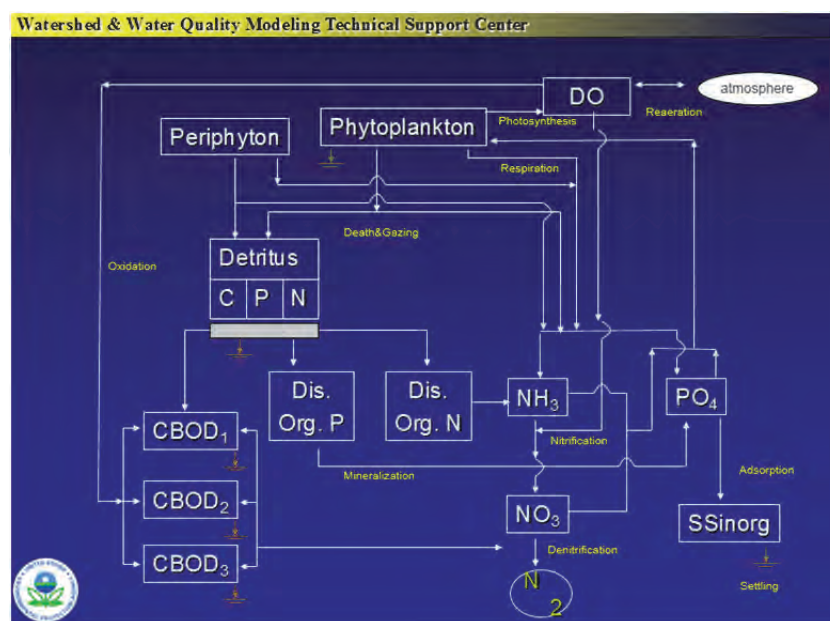
Fig. 2. Model for eutrophication used by WASP; source: USEPA [2015]
