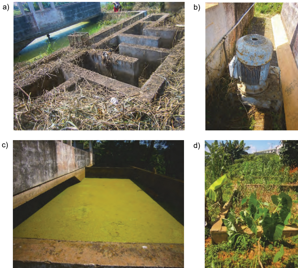
Photo 4. View of the abandoned treatment plant of CHU: a) pretreatment tank, b) turbine, c) aeration tank, d) sand bed; (phot. G.A. Ajeegah)
