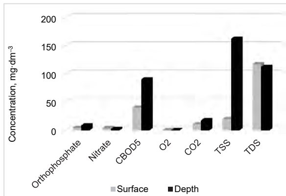
Fig. 4. Eutrophication parameters of Lake Obili; source: own study
