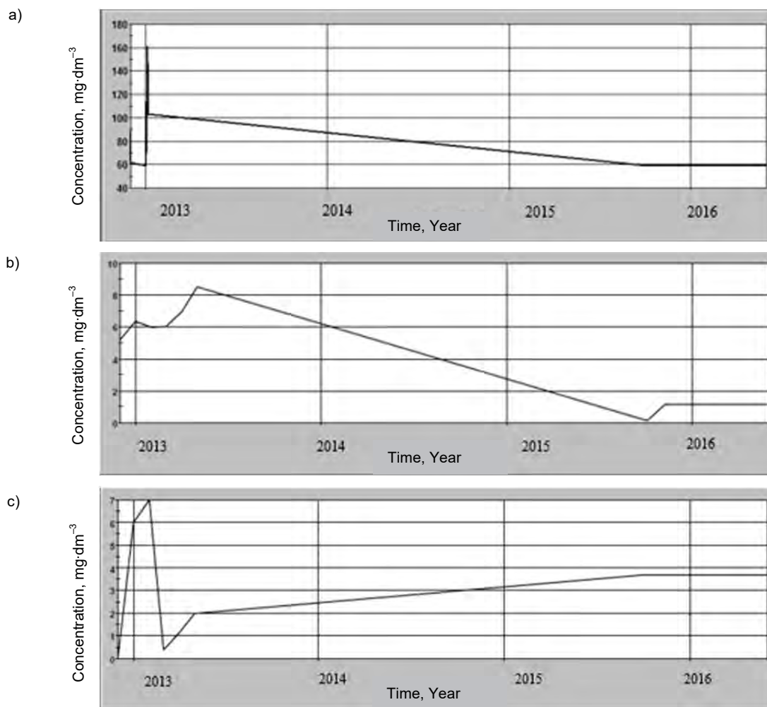
Fig. 6. Simulation of concentration measured and calculated by WASP: a) CBOD1U, b) DO, c) nitrate (NO 3 ); source: own study
