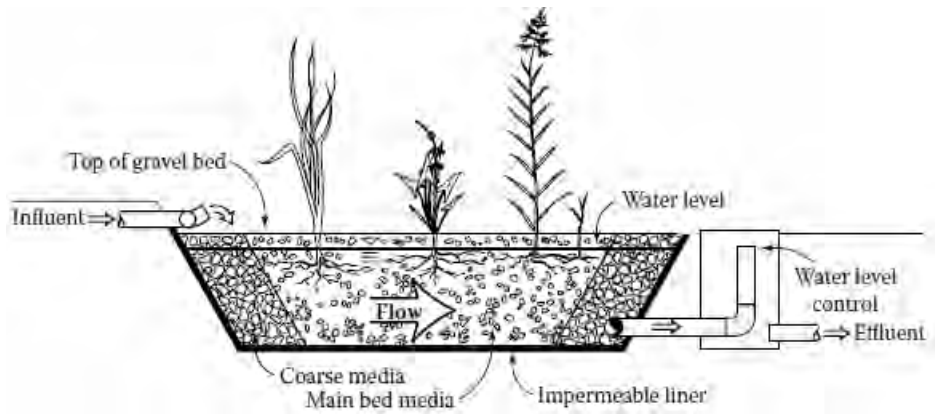
Fig. 12. Deep flow wetland; source: KADLEC and WALLACE [2009] adapted by Ajeegah et al
