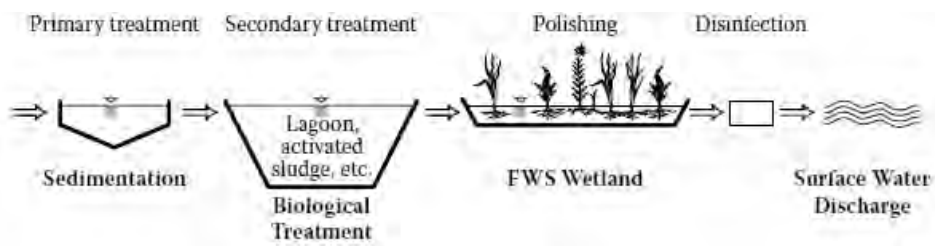
Fig. 11. Surface wetland and activated sludge; source: KADLEC and WALLACE [2009], modified
