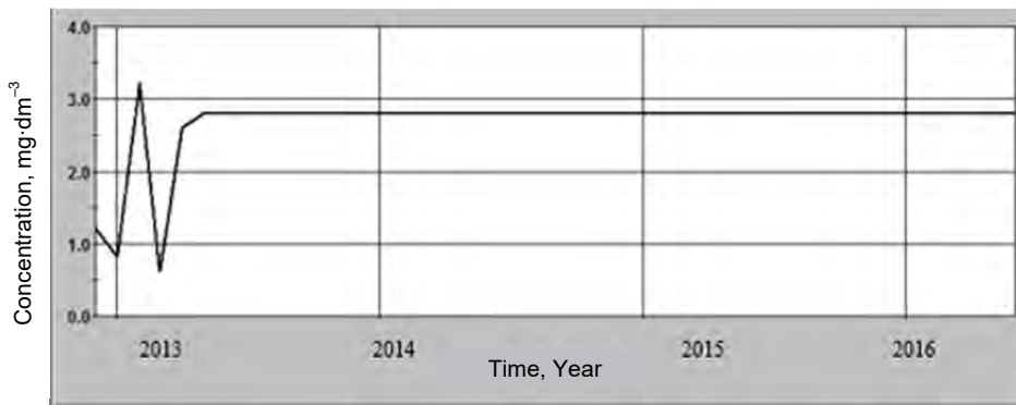
Fig. 5. Simulation of ammonia (NH 4 ) concentration measured and calculated by WASP; source: own study
