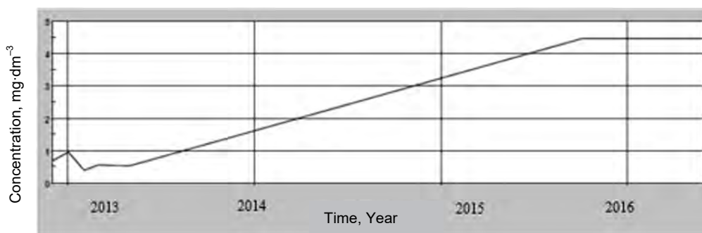
Fig. 7. Simulation of orthophosphate (OPO 4 ) by WASP measured and calculated with WASP; source: own study
