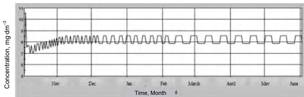
Fig. 8. Lake response after application of 45 t oxygen daily (DO) load measured and calculated with WASP; source: own study
