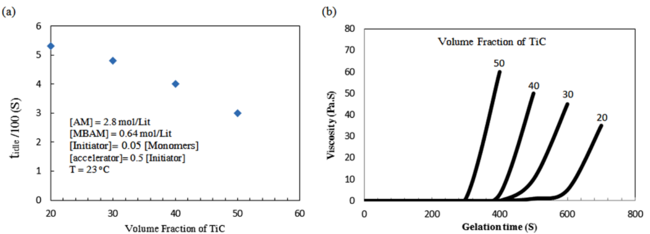
Fig. 9. (a) t_{idle} as a function of the ceramic loading and (b) apparent viscosity as a function of the gelation time
