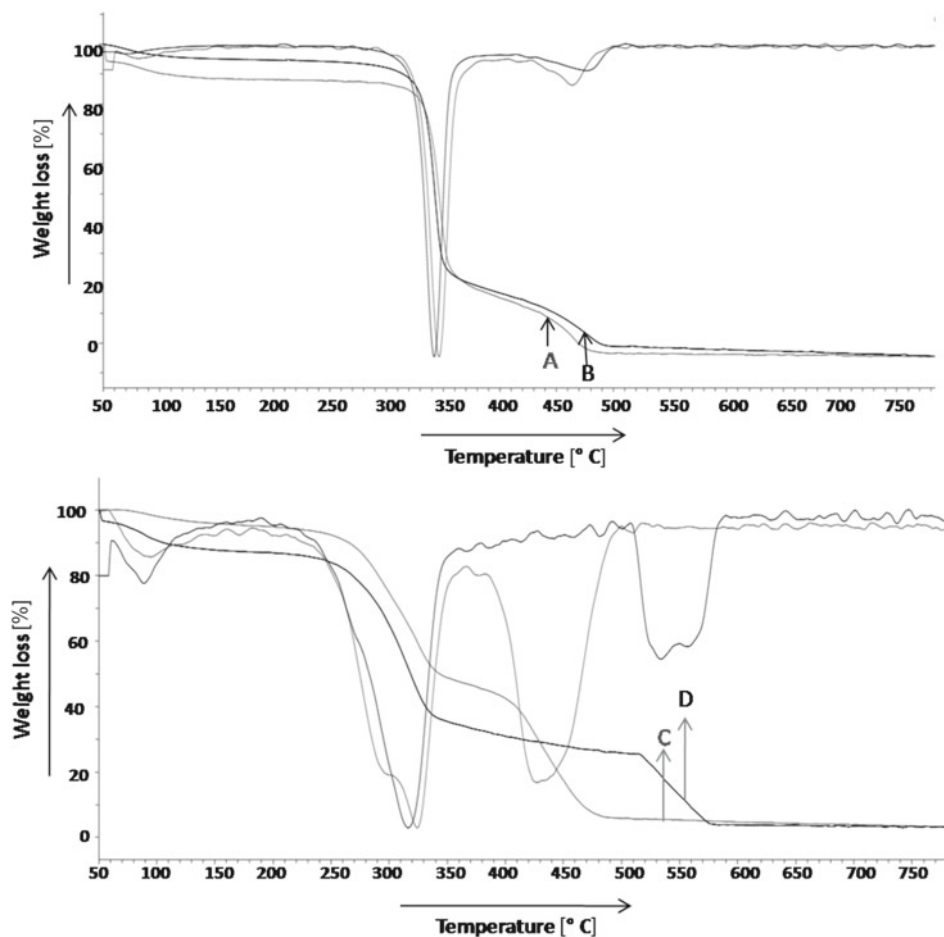
Figure 2. TGA curves of the Control (A), Mordanted (B), 1: 1 BPS treated (C) and 1: 0 BPS treated (D) cotton fabrics
