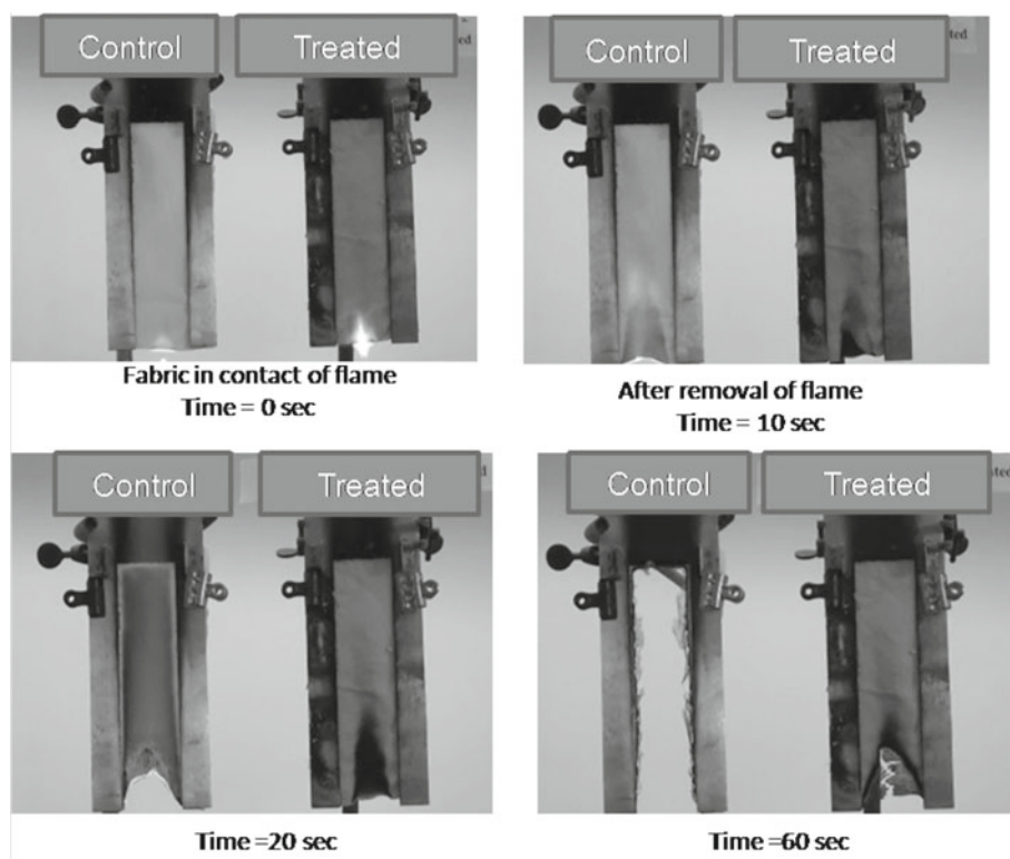
Figure 1. Comparison in burning behaviour of control and BPS treated (1: 0) cotton fabrics at different time interval
