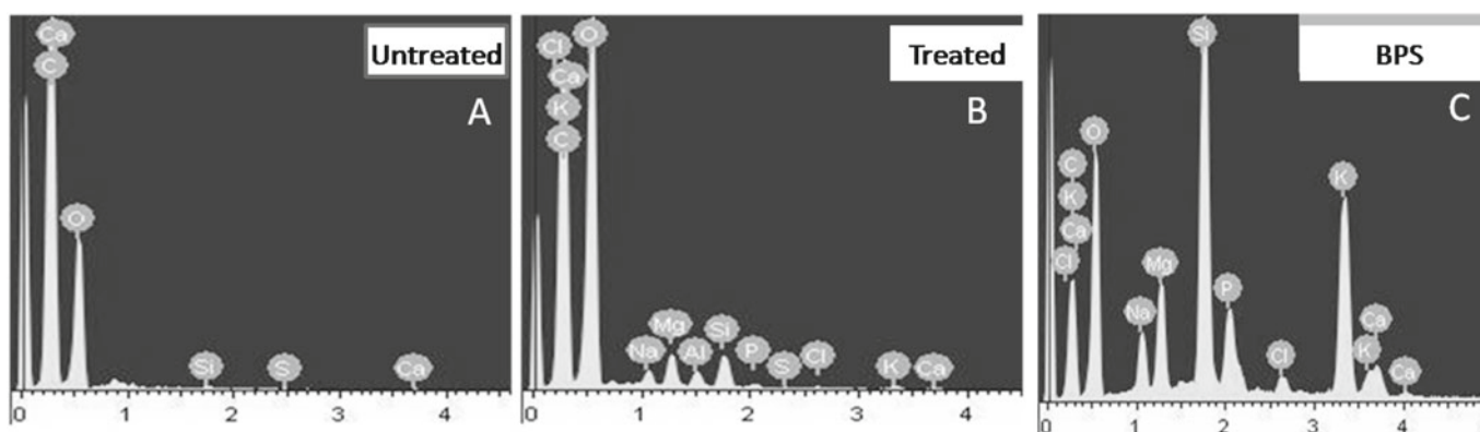
Figure 6. EDX images of untreated control (A), BPS treated (1:0) cotton fabrics (B) and BPS (C)
