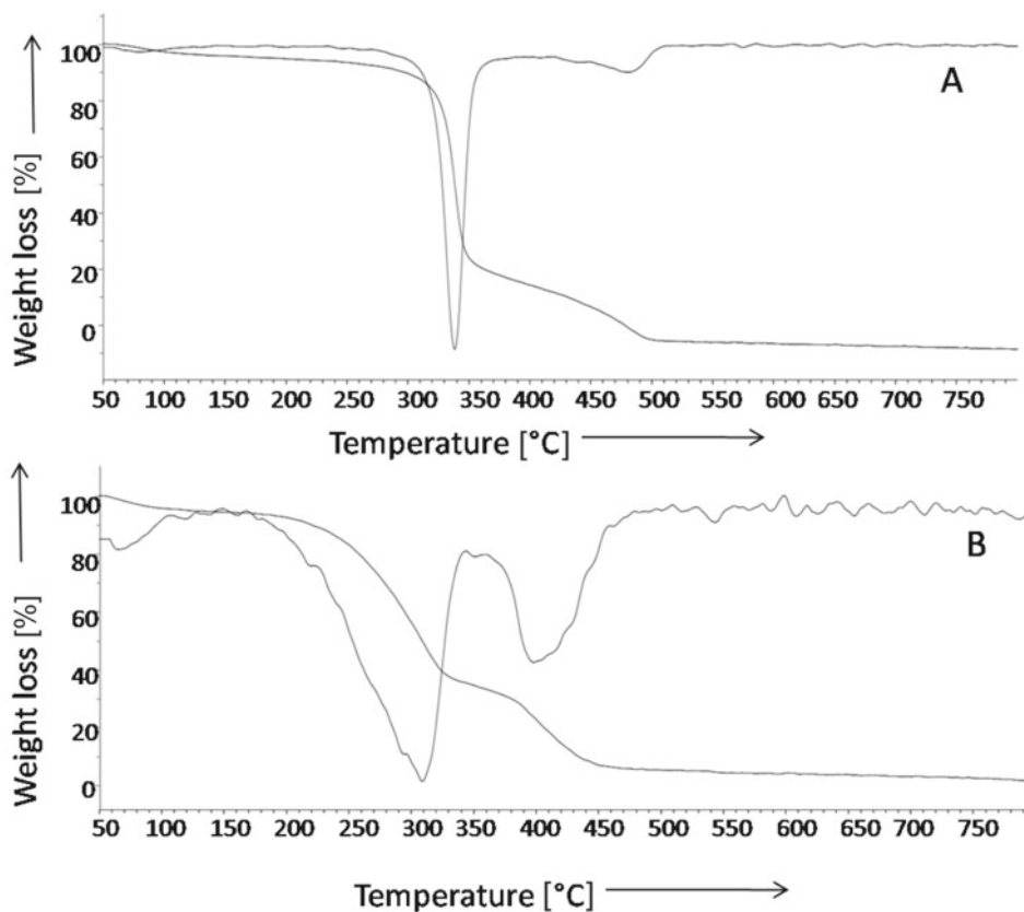
Figure 3. TGA curves of Control (A) and 1: 0 BPS treated (B) cotton fabrics
