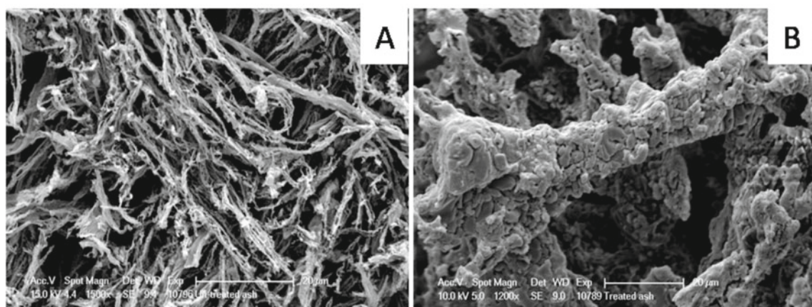
Figure 8. SEM of residual mass of control (A) and BPS treated (B) fabric
