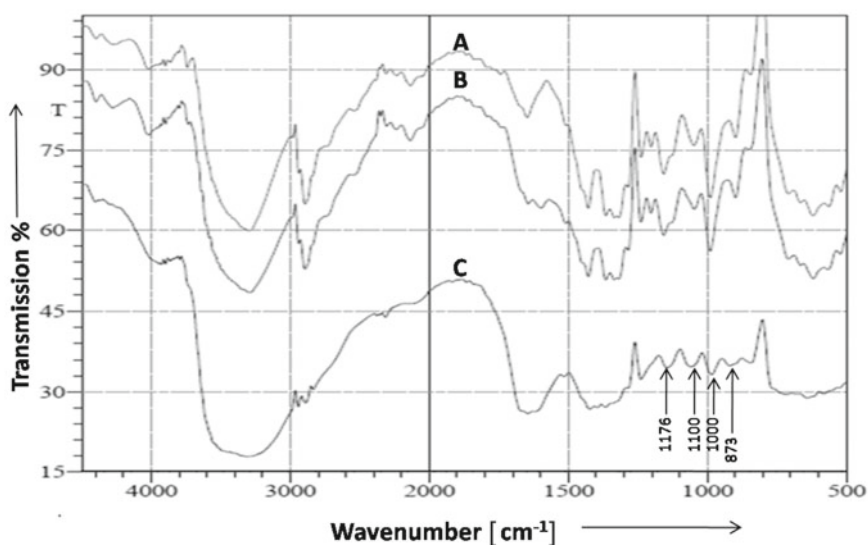
Figure 4. FTIR analysis of control fabric (A), BPS treated (1: 0) fabric (B) and dried BPS (C)
