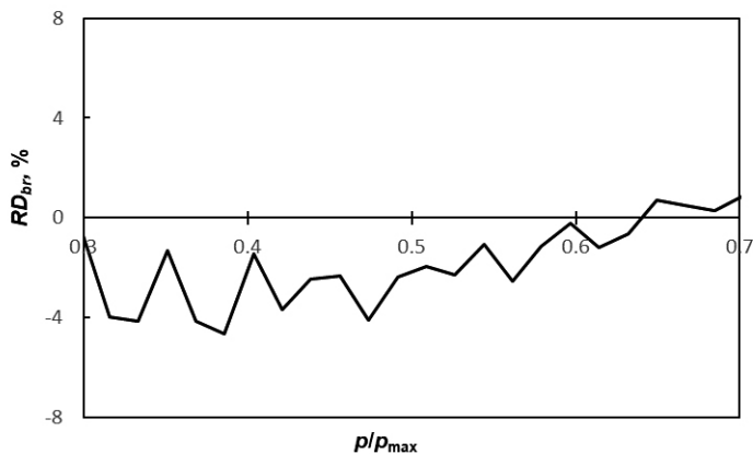
Figure 9. Relative difference in burning rate for the SC92 propellant
