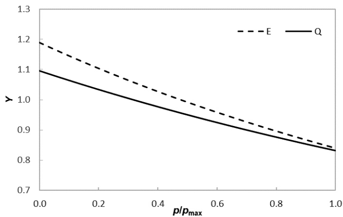
Figure 1. Y(p/p_{\max}) diagrams for 4/1 propellant for methods E and Q
