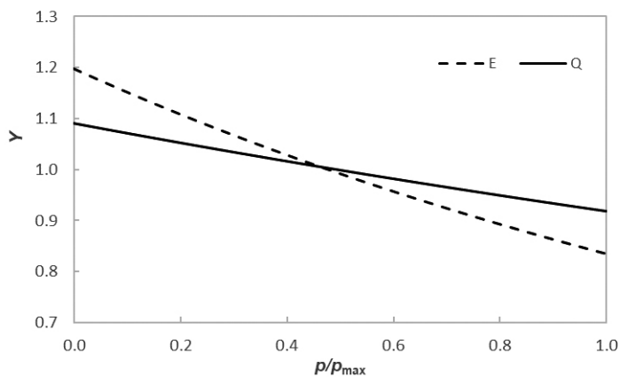
Figure 2. Y(p/p_{\max}) diagrams for JA-2 propellant for methods E and Q
