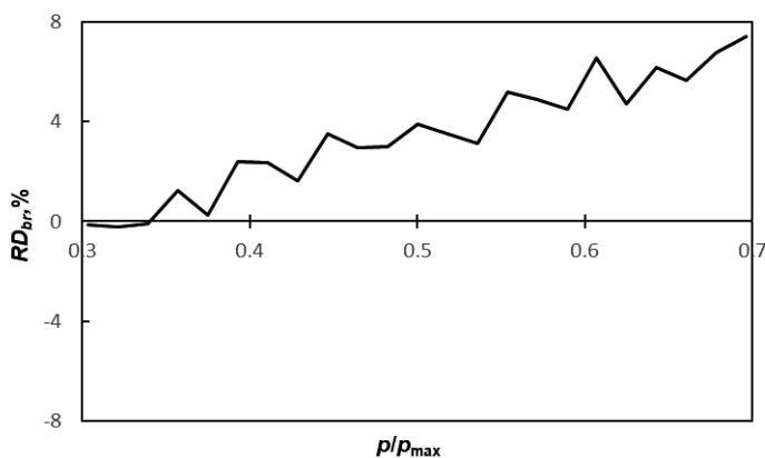
Figure 8. Relative difference in burning rate for the JA-2 propellant
