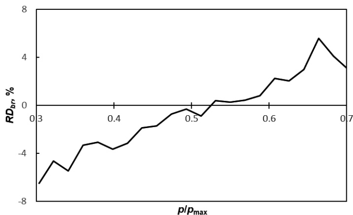
Figure 7. Relative difference in burning rate for the 4/1 propellant
