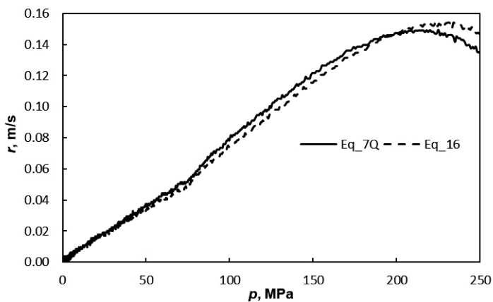
Figure 6. Diagrams r(p) for the SC92 propellant plotted on the basis of Equations 7 (method Q) and 16
