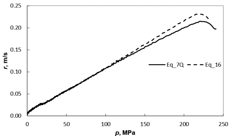
Figure 5. Diagrams r(p) for the JA-2 propellant plotted on the basis of Equations 7 (method Q) and 16
