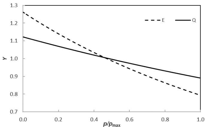
Figure 3. Y(p/p_{\max}) diagrams for SC92 propellant for methods E and Q
