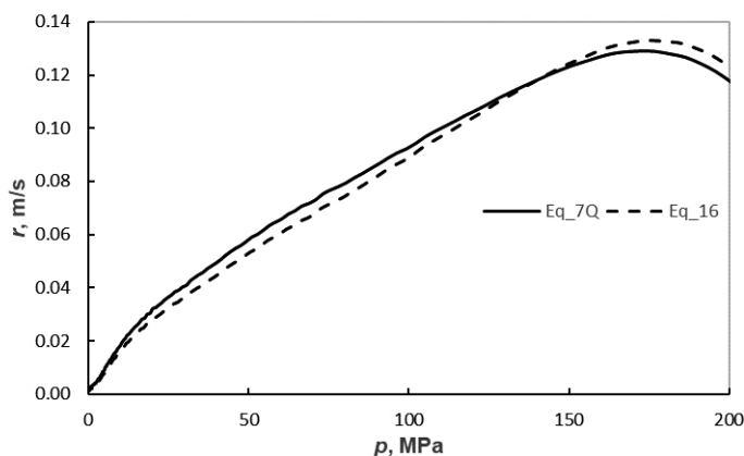
Figure 4. Diagrams r(p) for the 4/1 propellant plotted on the basis of Equations 7 (method Q) and 16
