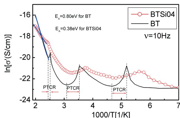
Fig.4. A plot of the a.c. conductivity ( \sigma' ) in the Arrhenius system with frequency measurement field of 10 Hz for BTSi04 and BT samples
