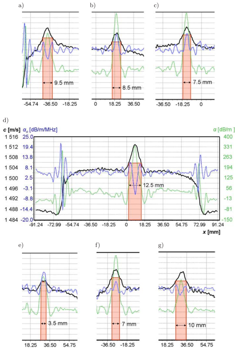
Fig. 11. Pixel value distributions for the lines indicated in Fig. 10, along the diameters of individual phantom inclusions, drawn in turn for 3 different UTT images (see Fig. 6), the ultrasound velocity – black colour, derivative of ultrasound attenuation coefficient in relation to frequency – blue colour, ultrasound attenuation coefficient – green colour: a) d_{inc1} = 9.5 mm, b) d_{inc2} = 8.5 mm, c) d_{inc3} = 7.5 mm, d) d_{inc4} = 12.5 mm, e) d_{inc5} = 3.5 mm, f) d_{inc6} = 7 mm, g) d_{inc7} = 10 mm.
