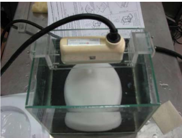
Fig. 4. US measurement methodology – a view of the tank.
