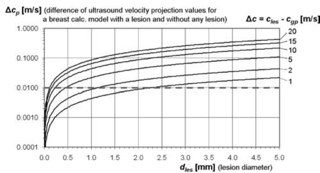
Fig. 12. Calculations of the difference of ultrasound velocity projection values for a breast calculation model with a lesion and without any lesion, depending on the lesion diameter, with the parameter \Delta c = 1, 2, 5, 10, 15, 20 m/s.
