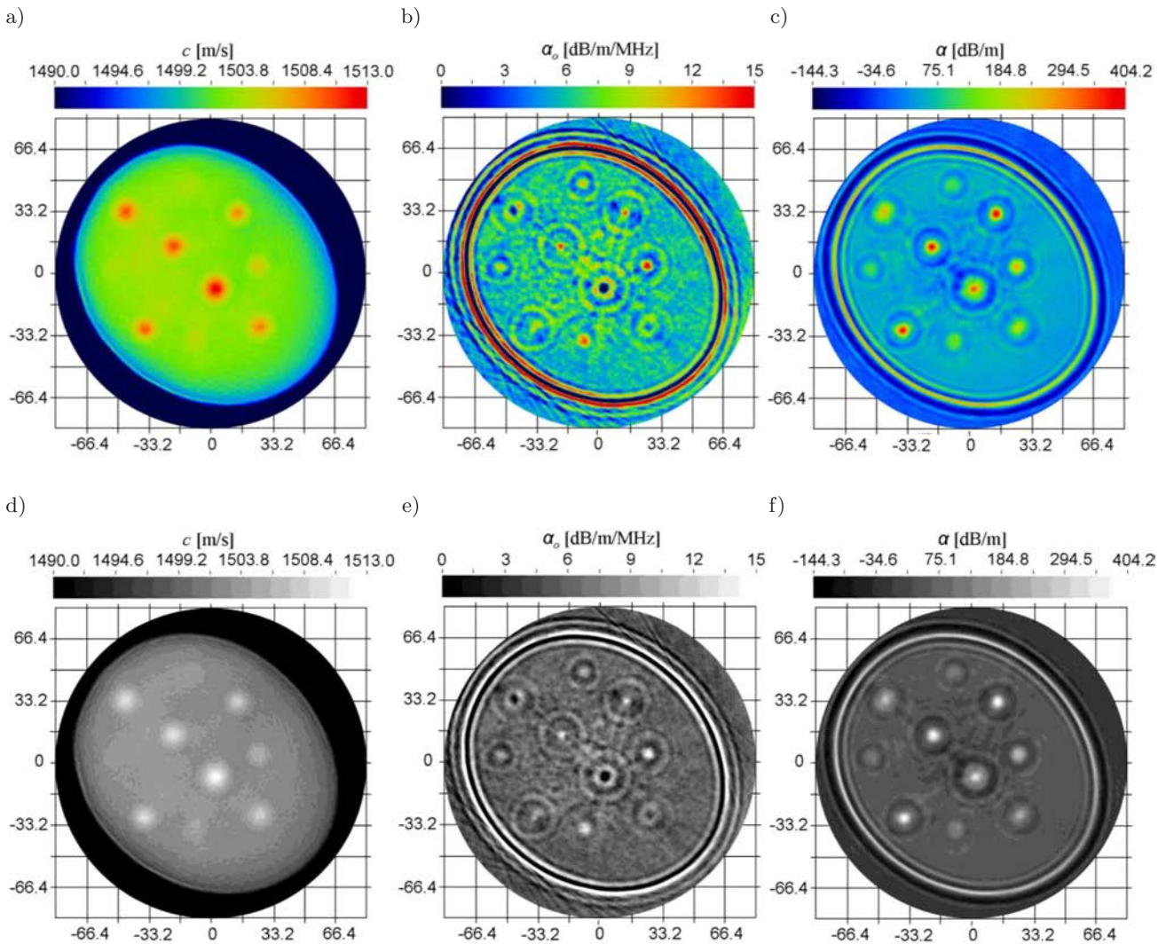
Fig. 6. UTT images of the CIRS Model 059 phantom longitudinal cross-section at the height of z = 20 mm (presented in rainbow colours and greyscale): a), d) ultrasound propagation velocity, b), e) derivative of the ultrasound attenuation coefficient in relation to frequency, c), f) the ultrasound attenuation coefficient.
