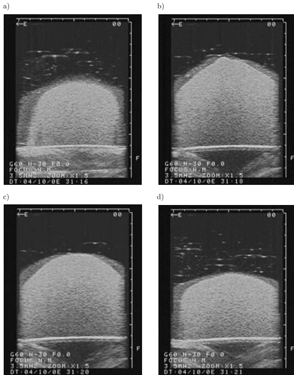
Fig. 7. Examples of US images of transverse cross-sections of the CIRS Model 059 phantom for the following distances of the linear probe axis from the edge of the tank (where inclusions expected): a) 2 cm, b) 5.5 cm, c) 7.5 cm, d) 11 cm.
