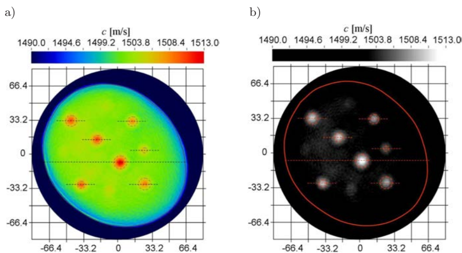
Fig. 10. UTT image of distribution of local values of ultrasound velocity for the CIRS Model 059 phantom longitudinal cross-section for the height of z = 20 mm, with contours of the shape of the cross-section and inclusion edges rendered from a CT image (Fig. 8b): a) rainbow colours image, b) greyscale image with boosted contrast ( 50 \rightarrow 80\% ) and reduced brightness ( 50 \rightarrow 32\% ).
