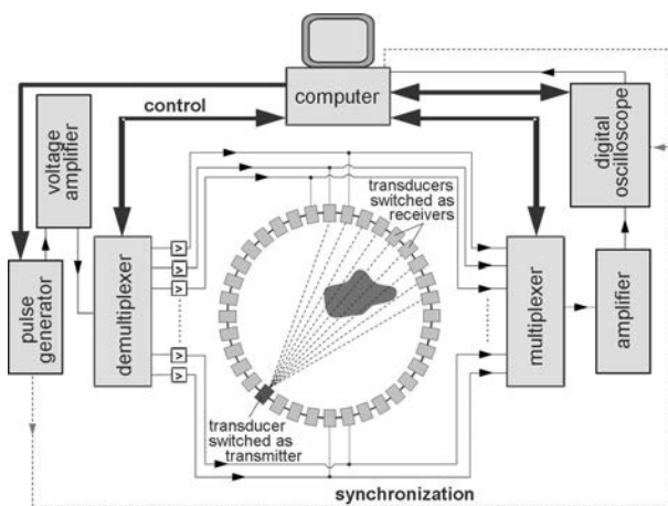
Fig. 1. Simplified block diagram of the measurement research stand for UTT with the ring probe.
