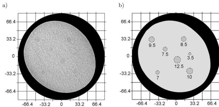
Fig. 8. CT image of the CIRS Model 059 phantom longitudinal cross-section for the height of z = 20 mm: a) increased contrast image, b) estimation of the size of distinguishable heterogeneous areas using an edge rendering image method.
