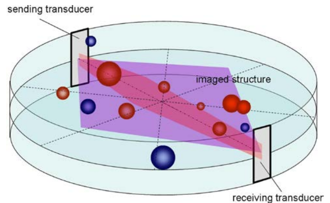
Fig. 13. Exemplary representation of the location of inclusions in the examined structure for the measurement space whose height is equal to the height of the elementary ultrasonic transducers of a ring probe (red inclusions are located in the horizontal plane of the transducer's axis).
