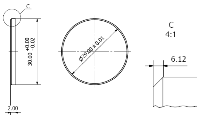
Fig. 1. Specimen geometry (dimensions in mm)
