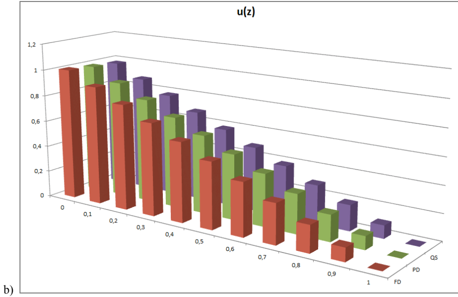
Fig. 5. Skeleton and fluid displacement for Biot's, u-p and consolidation model for \eta = 0.1
