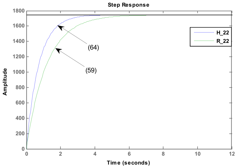
Figure 10: Step responses of H_{22} and R_{22}
