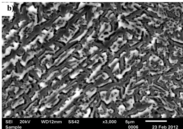
Fig. 4. Microstructures of cast steel: a) GX2CrNiMoN25-6-3 1120°C/water+800°C/180min, b) GX2CrNiMoCuN25-6-3-3 1120°C/water + 800°C/180min
