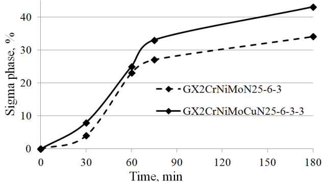
Fig. 3. The kinetics of \sigma phase precipitation at a temperature of 800°C
