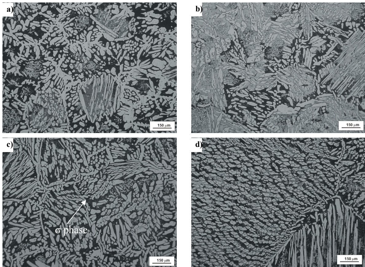
Fig. 2. Microstructures of cast steel: GX2CrNiMoCuN25-6-3-3 a) 1120°C/water+800°C/75min, c) 1120°C/water + 800°C/180min, GX2CrNiMoN25-6-3 b) 1120°C/water + 800°C/75min, d) 1120°C/water + 800°C/180min
