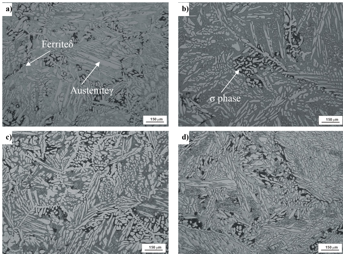
Fig. 1. Microstructures of cast steel: GX2CrNiMoCuN25-6-3-3 a) 1120°C/water+800°C/30min, c) 1120°C/water + 800°C/60min, GX2CrNiMoN25-6-3 b) 1120°C/water + 800°C/30min, d) 1120°C/water + 800°C/60min
